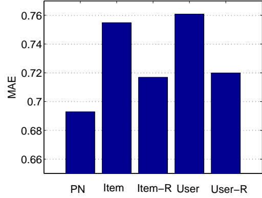
Figure 4: The mean absolute error of recommendation methods (Item: item-based method, Item-R: item-based method with rounding, User: user-based method, and User-R: user-based method with rounding).
