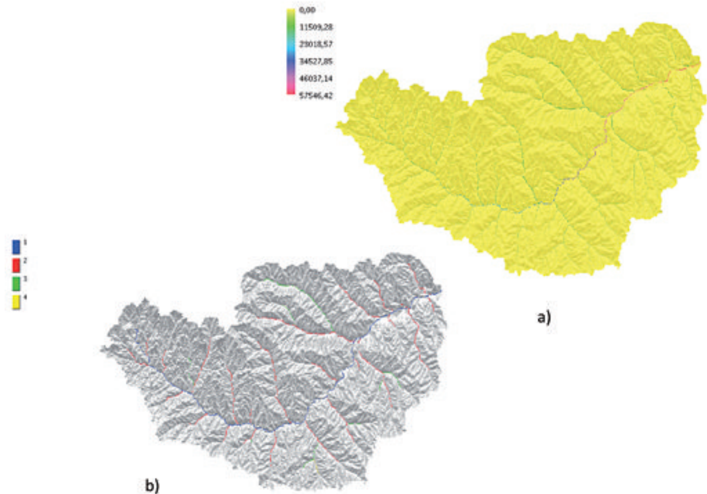
Figure 4. The Little Washita basin: output of HackLength, (a), and Hack Stream, (b). Figura 4. La cuenca Little Washita: (a) salida HackLength y (b) salida de Hack Stream.
