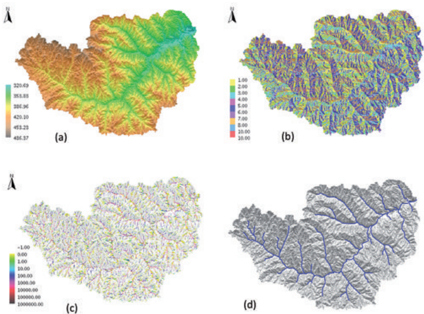
Figure 2. The Little Washita basin: output of the Pitfiller Horton Machine (a), DrainDir, (b) TCA (c) and Extract Network (d). Figura 2. La cuenca Little Washita: (a) salida de la Máquina Pitfiller Horton; (b) DrainDir; (c) TCA y (d) Extract Network.
