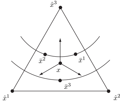
Figure 2: Semi-simple solution under (C2)
