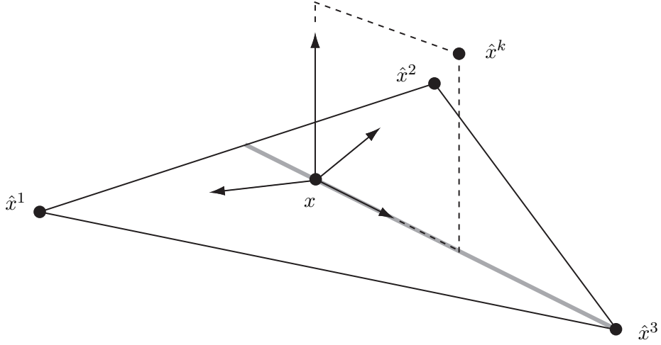
Figure 3: Part (iv) of Condition (C2)
