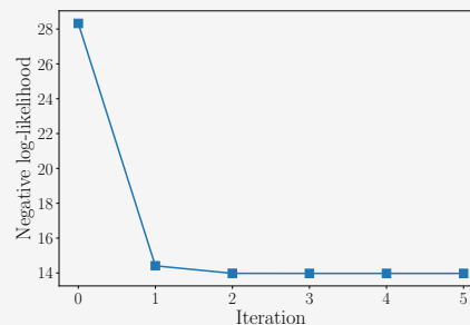
(b) Negative log-likelihood as a function of the EM iterations.
