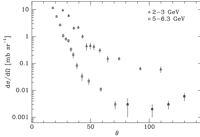
Figure 12.2 The differential cross-section for neutron-proton scattering at two values of the centre-of-mass energy. Data obtained from M. Kreisler et al. , Phys. Rev. Lett., 16 , 1217, (1966). The diffraction peak at \theta = 0 can be understood in terms of the optical theorem.
