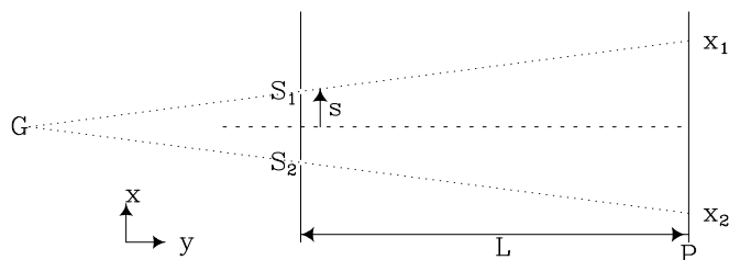
Figure 1.1 The two-slit interference experiment.
