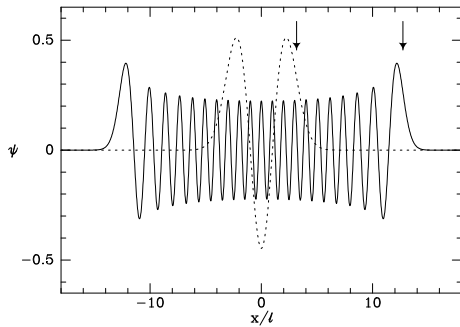
Figure 3.5 The wavefunctions \langle x|2\rangle and \langle x|40\rangle of two stationary states of a harmonic oscillator.
