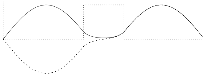
Figure 5.8 The ground state (full curve) and the associated odd-parity state (dashed curve) of the double square-well potential (shown dotted).
