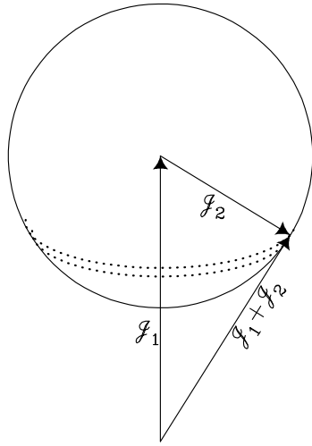
Figure 7.14 Classically the sum vector \mathcal{J}_1 + \mathcal{J}_2 can line anywhere on the sphere of radius |\mathcal{J}_2| around the end of \mathcal{J}_1 .
