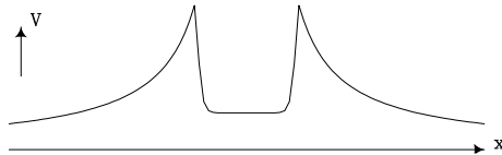
Figure 5.15 Schematic of the potential-energy function V(x) experienced by an \alpha -particle near an atomic nucleus. The short-range ‘strong’ force causes the particle’s potential energy to rise extremely steeply at the edge of the nucleus. The long-range electrostatic repulsion between the nucleus and the alpha particle causes V(x) to drop steadily as the \alpha -particle moves away from the nucleus.
