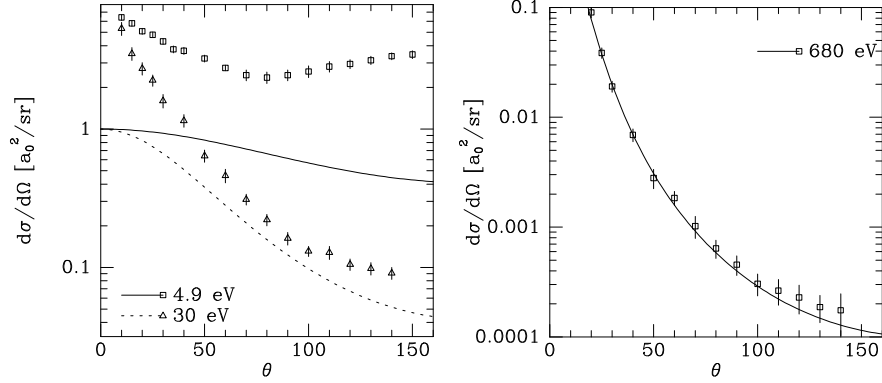
Figure 12.4 Elastic e^- -H scattering at electron kinetic energies E = 4.9, 30 and 680 eV. The curves show the predictions of the Born approximation (eq. 12.75) while the points show experimental data from J.F. Williams, J. Phys. B , 8 no. 13 (1975). The accuracy of the Born approximation increases with energy.
