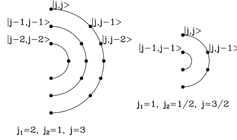
Figure 7.12 The left panel shows states obtained by adding a system of angular momentum j_2 = 1 to one with j_1 = 2 , while the right panel is for j_1 = 1 and j_2 = \frac{1}{2} .
