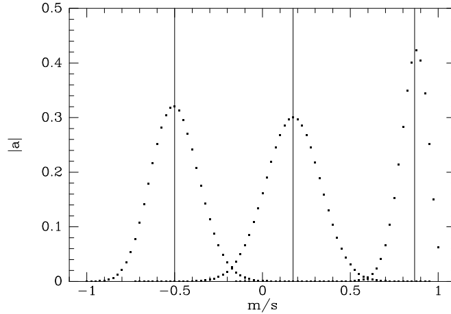
Figure 7.11 The points show the absolute values of the amplitudes a_m \equiv \langle s, m, z | s, s, \theta \rangle for s = 40 and, from left to right, \theta = 120^\circ, 80^\circ, 30^\circ . For each value of \theta , the vertical line shows the value of \cos \theta .
