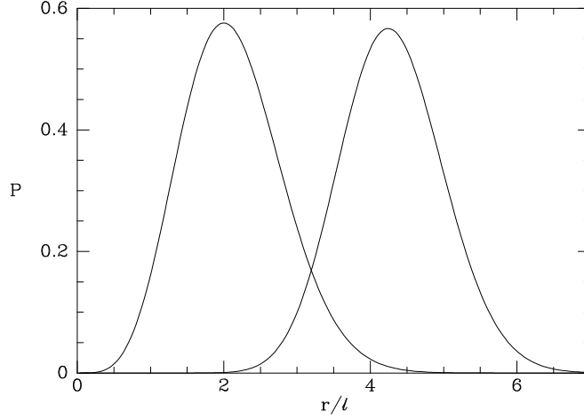
Figure 7.7 Radial probability distributions of circular orbits in the three-dimensional harmonic oscillator potential for \mathcal{L} = 1 and \mathcal{L} = 8 . The scale radius \ell = \sqrt{\hbar/2m\omega} .
