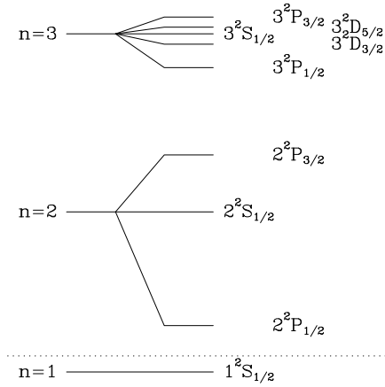
Figure 8.6 The fine structure of a hydrogen-like ion with Z = 200 that is predicted by equation (8.76a). The dotted line denotes a break in the energy scale so that the ground state can be included.
