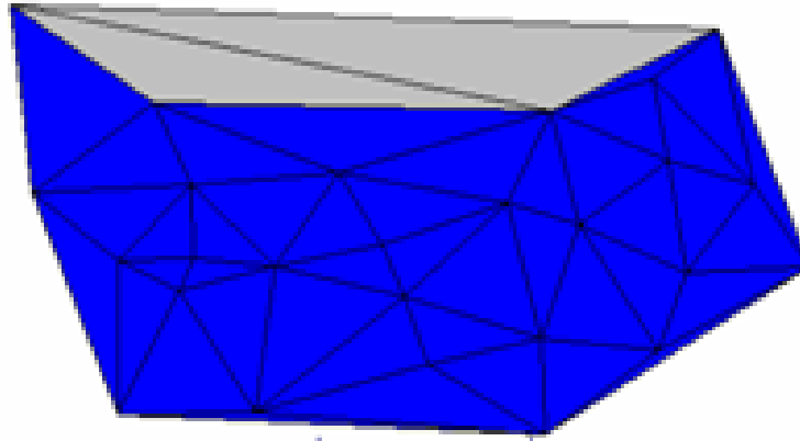
Figure 1. Illustration of \alpha -hull. The lines show the Delaunay triangulation (the intersection points of the lines are the species' or ecological community's occurrence locations). The sum of the areas of darker triangles is range extent based on the \alpha -hull. The two lighter colored triangles that are part of the convex hull are excluded from the \alpha -hull. (IUCN Standards and Petitions Working Group 2008)
