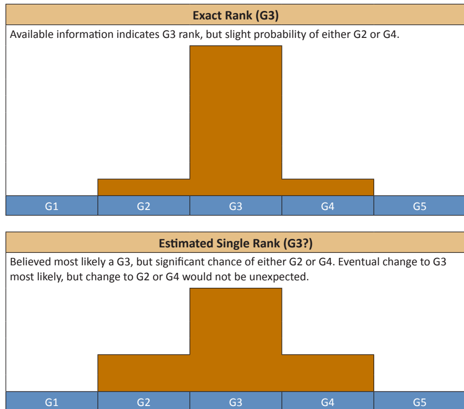
Figure 3. Comparison of uncertainty associated with examples of an exact status rank, rank with “?” qualifier, and range ranks.
