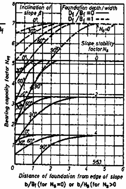
(e) Cohesive Soil ( \phi=0 )
