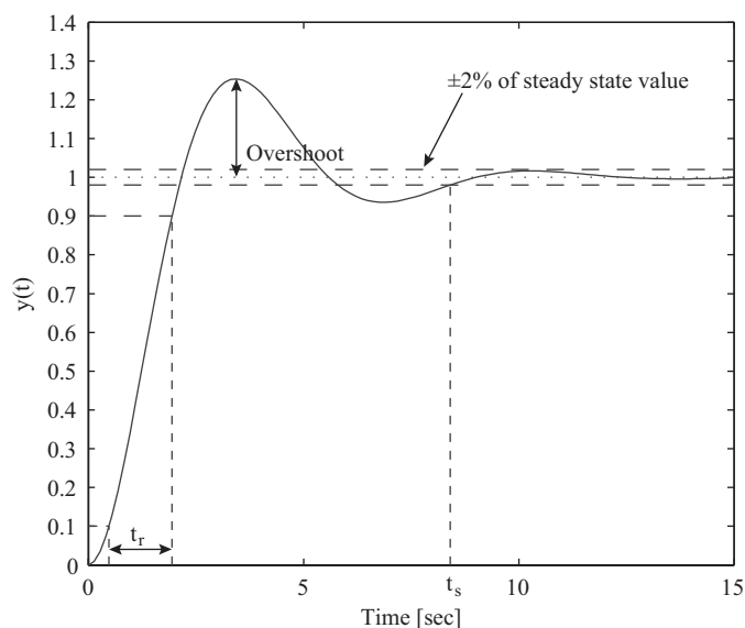
FIGURE 2.10: Characteristic parameters of the step response of a second order system.
