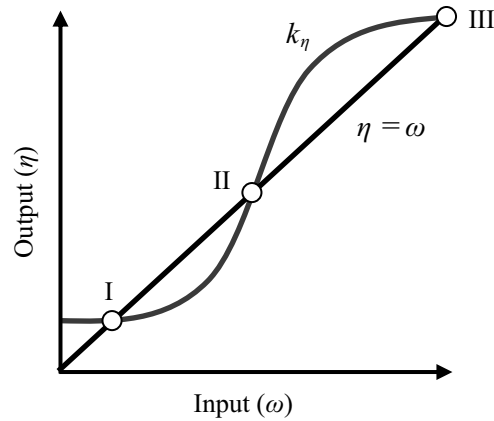
FIGURE 5.6: The sigmoidal steady-state I/O static characteristic curve k_\eta has three intersections with the line representing \omega as a function of \eta for unitary positive feedback. The three intersection points (I, II, and III) represent two stable steady-states (I and III) and one unstable steady-state (II) for the closed-loop system.
