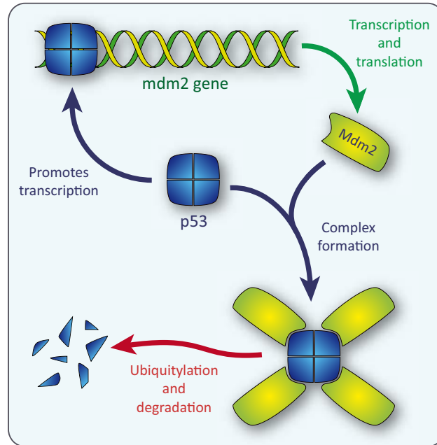
FIGURE 4.11: Biochemical interactions between p53 and Mdm2.
