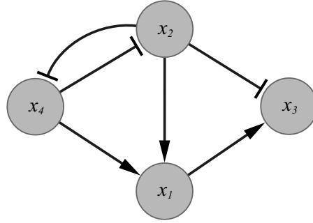
FIGURE 7.2: Toy network used in the examples. The shape of the arrow ending indicates the effect on the target node: \Delta and \top shapes are used for positive and negative effects, respectively (e.g. induction or repression of transcription of a gene).
