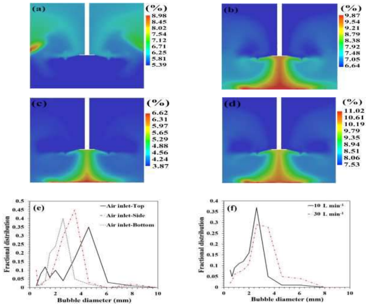
Fig. 5: The \alpha_G profiles with air inlet place on side (a) and at the bottom (b), and air flow rates of 10 L/min (c) and 30 L/min (d), as well as F_b under various air inlet locations (e) and air flow rates (f).
