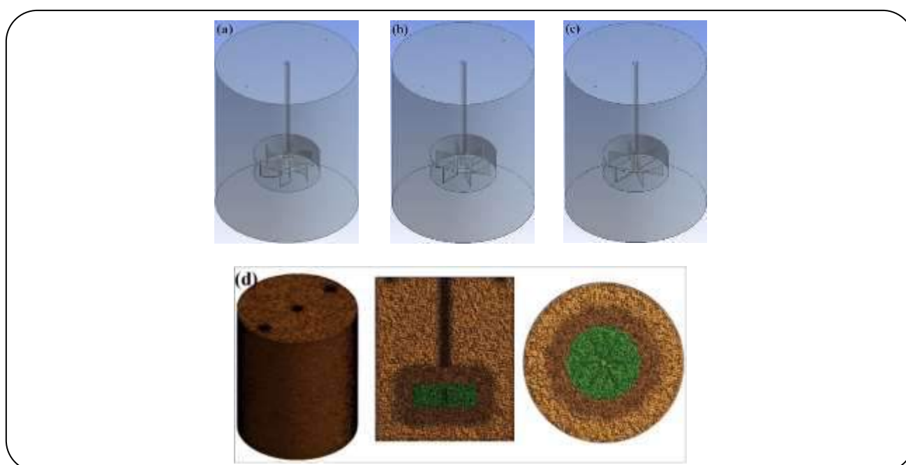
Fig. 1 Geometric models of the bioreactor with CBDT (a), RT (b), and PT (c) impellers, and computational grids of the bioreactor equipped with CBDT impeller (d).
