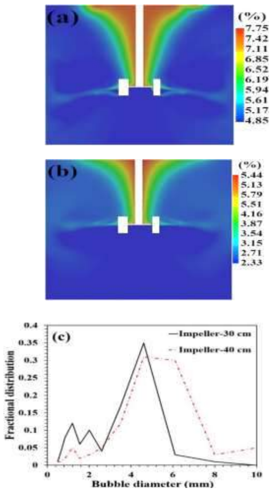
Fig. 4: The \alpha_G profiles with the impeller location in 30 cm (a) and 40 cm (b), and F_b at different location of impeller (c).
