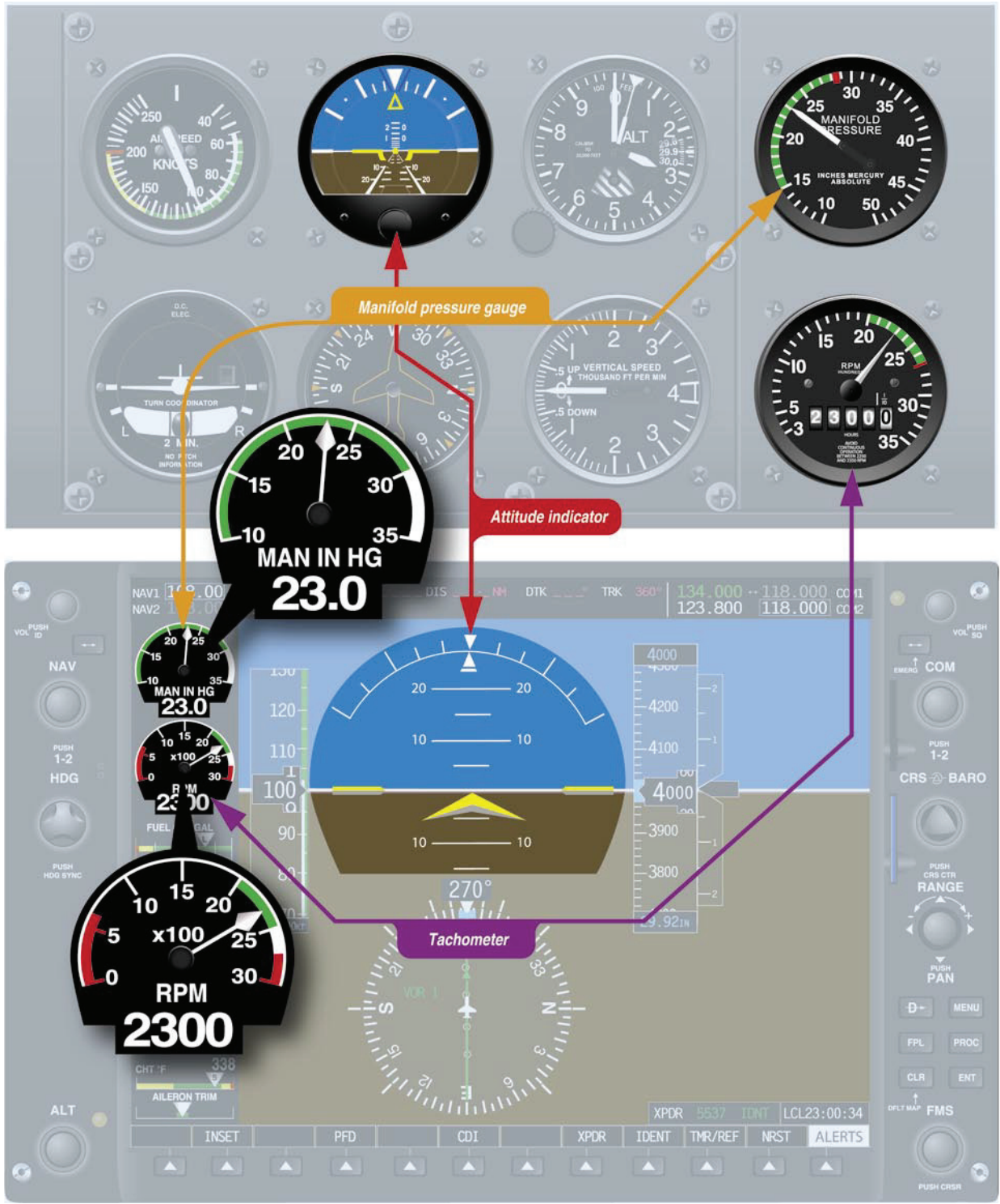
Figure 2-20. Control instruments.
