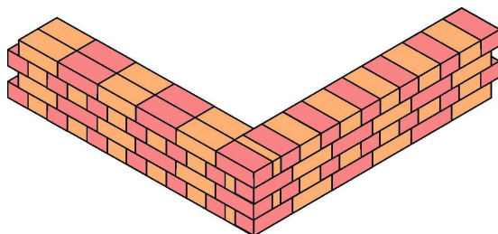
English bond
