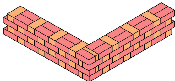
Flemish bond
