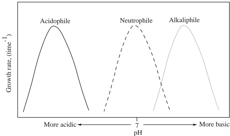
Figure 4.4: Growth rate versus pH for three environmental classes of procaryotes. Most free-living bacteria grow over a pH range of about three units. Note the symmetry of the curves below and above the optimum pH for growth.
