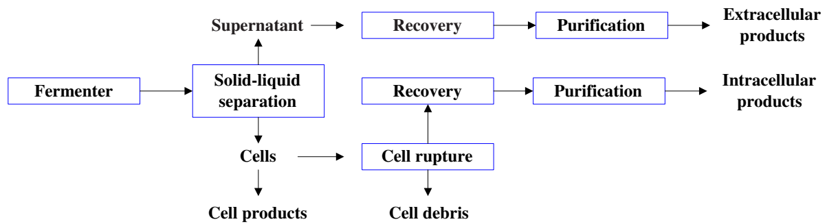
Figure 13.1: Major process steps in downstream processing.
