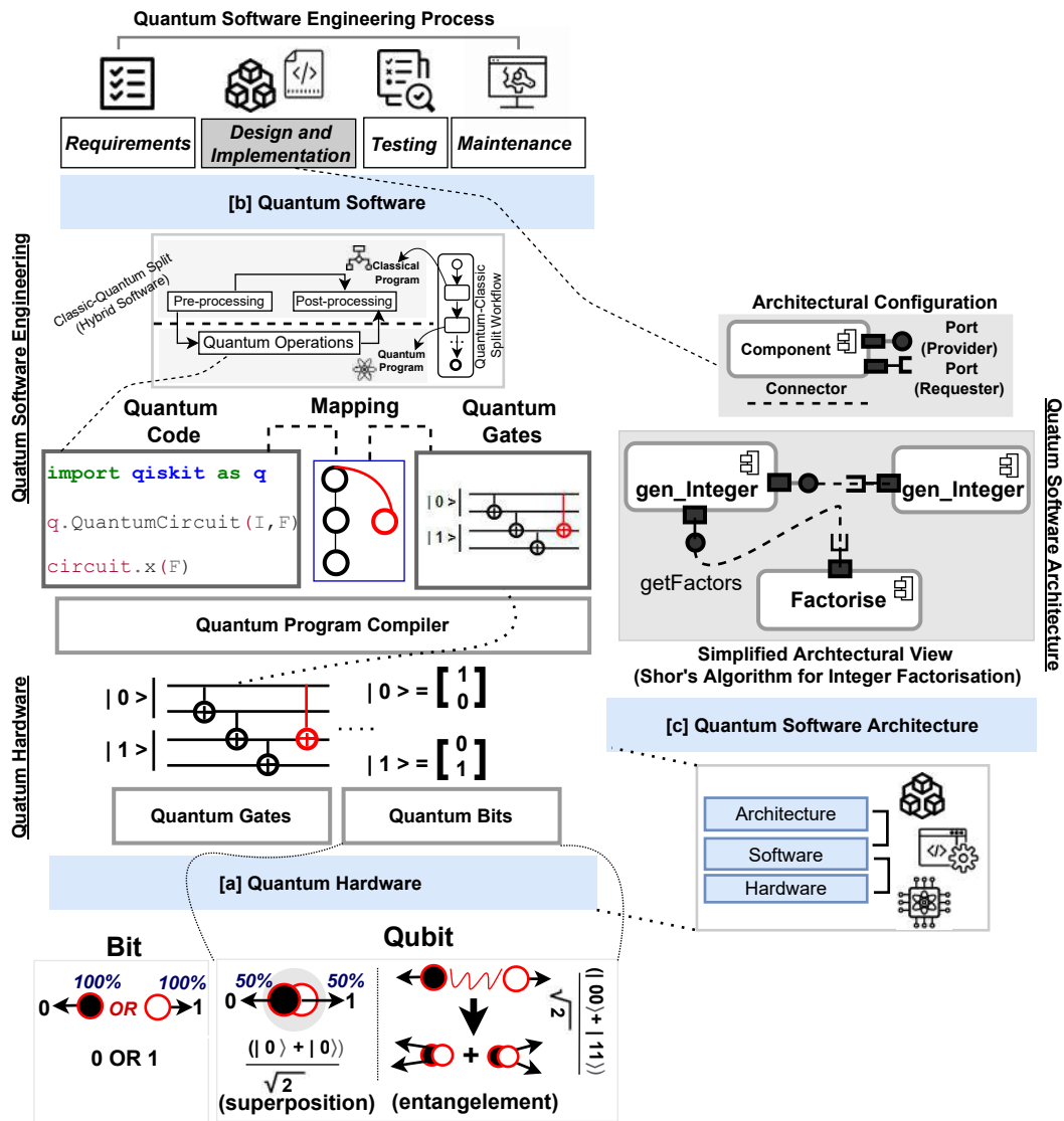
Figure 1: A Simplified View of Quantum Computing Systems ([a] Quantum Hardware, [b] Quantum Software, [c] Quantum Software Architecture)
