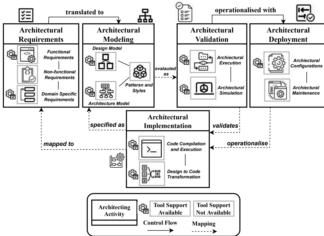
Figure 8: Tool support for architecting activities
