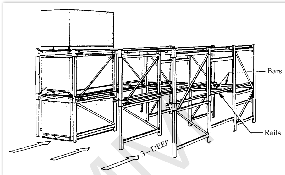
FIGURE 8: Drive-in Rack
