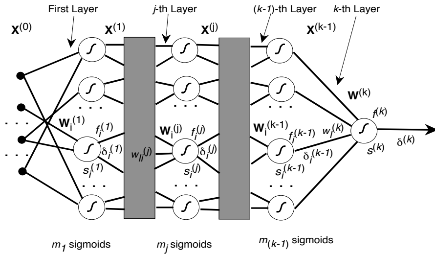
Figure 4.19: A Network with Sigmoid Units
