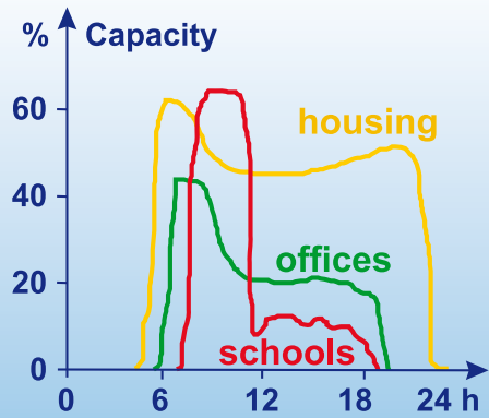
Variations in heating requirements during the day. 1
