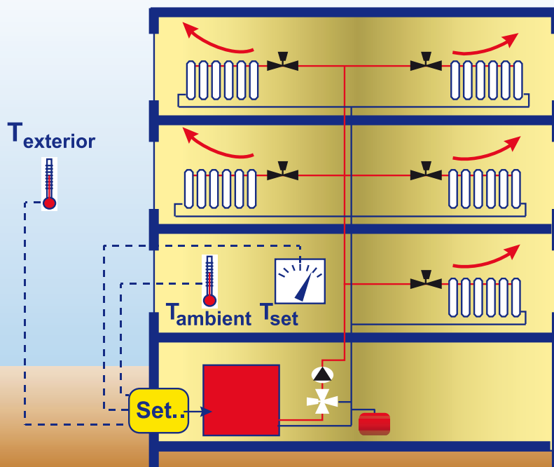
2 Functional diagram of a heating system with an exterior sensor, central thermostat and thermostatic radiator valves.
