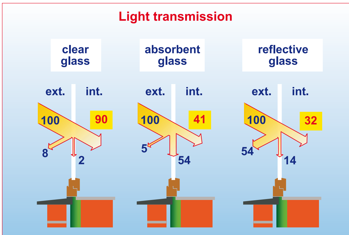
2 Light transmission for single glazing.
