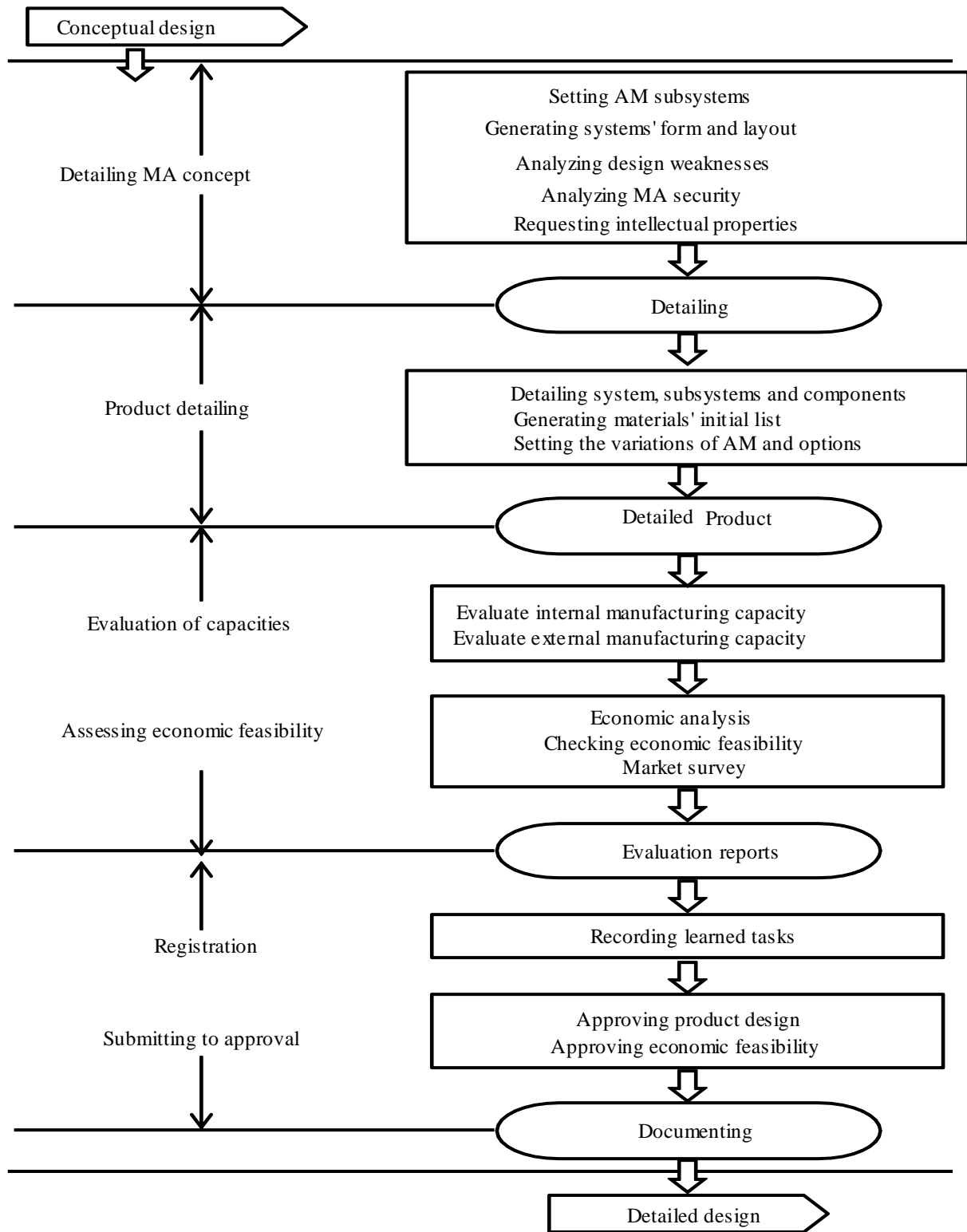
FIGURE 4. Scheme of the preliminary design phase.
