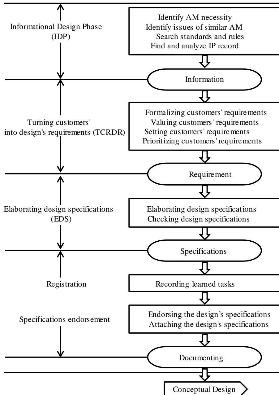
FIGURE 2. Scheme of the informational design phase.
