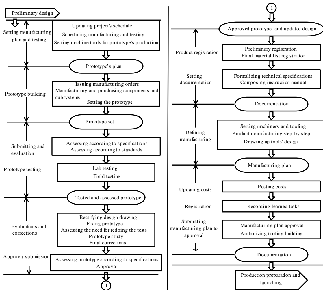
FIGURE 5. Scheme of the detailed design phase.
