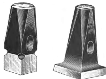
Set & Flatter
