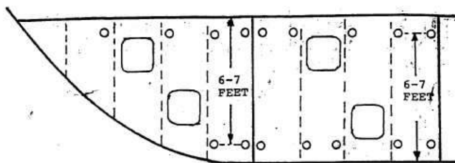
STAGING PIPE HOLES IN DOUBLE BOTTOM FLOORS
