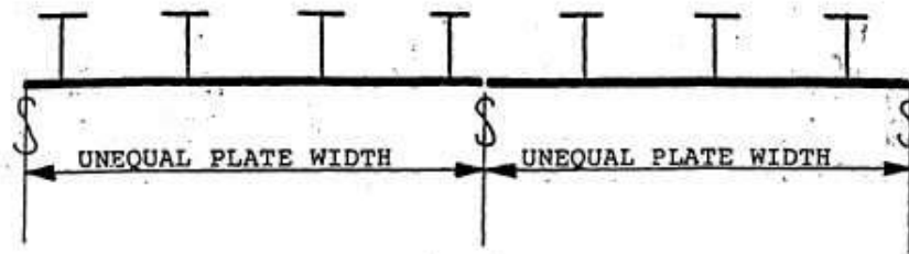
[A] NON-STANDARD PLATE WIDTH AND NUMBER OF STIFFENERS
