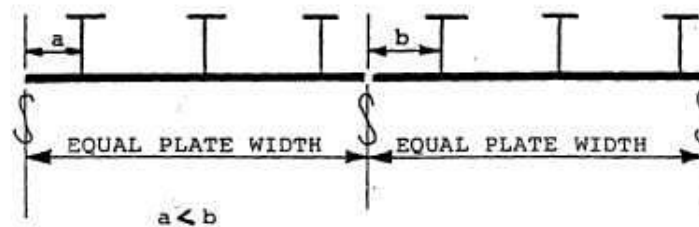
[B] ALSO NON-STANDARD DUE TO DIFFERENT STIFFENER MARKING
