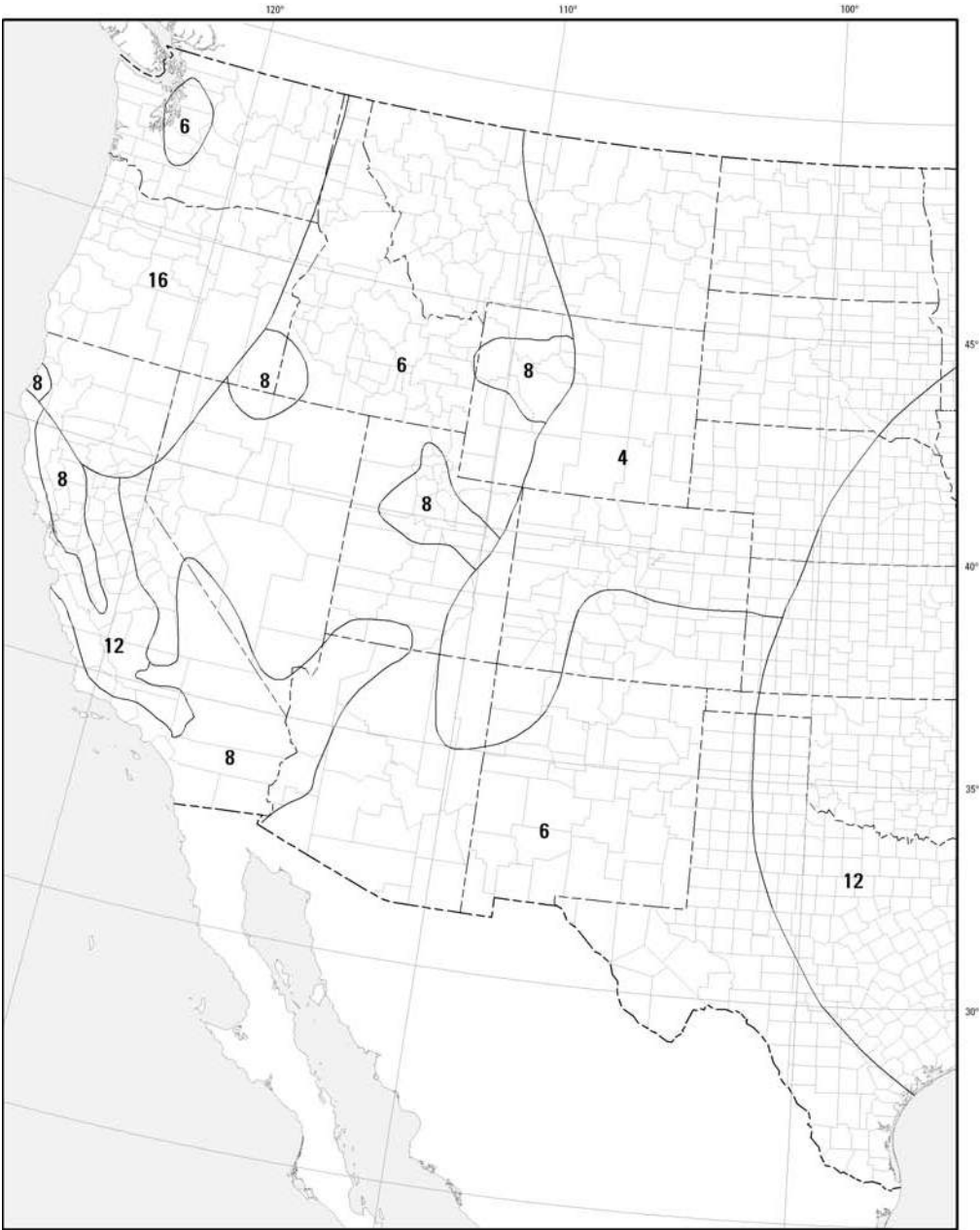
Figure 31 Map of long-period transition period, T_s , for the continental United States.
