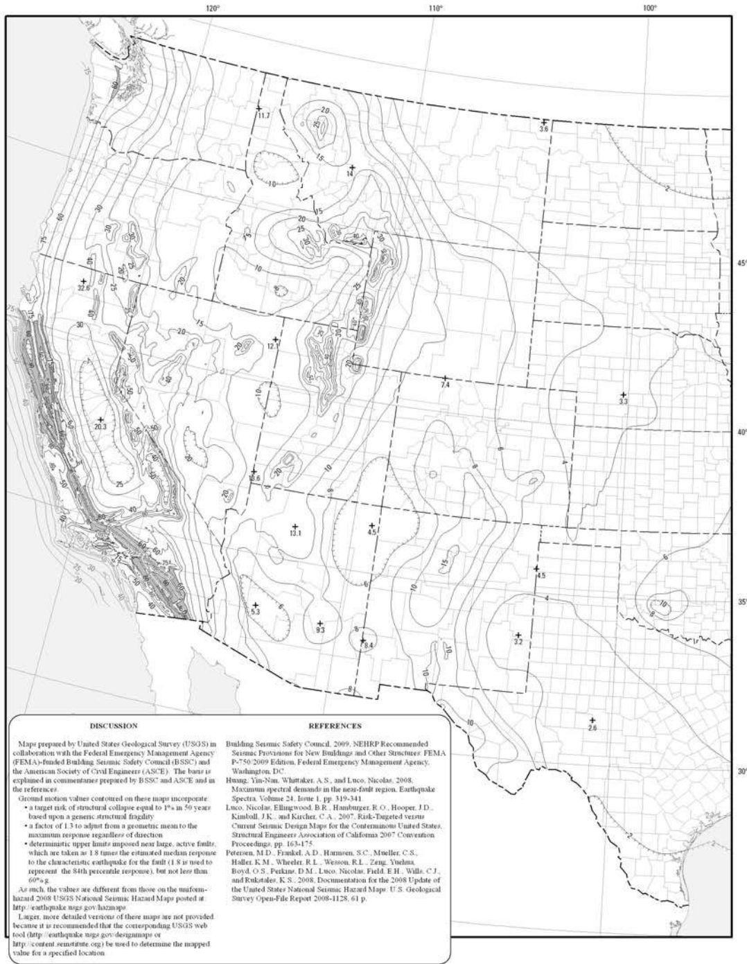
Figure 15 Distribution of 1-second period risk-targeted maximum considered earthquake response acceleration, S_1 , for the conterminous United States.
