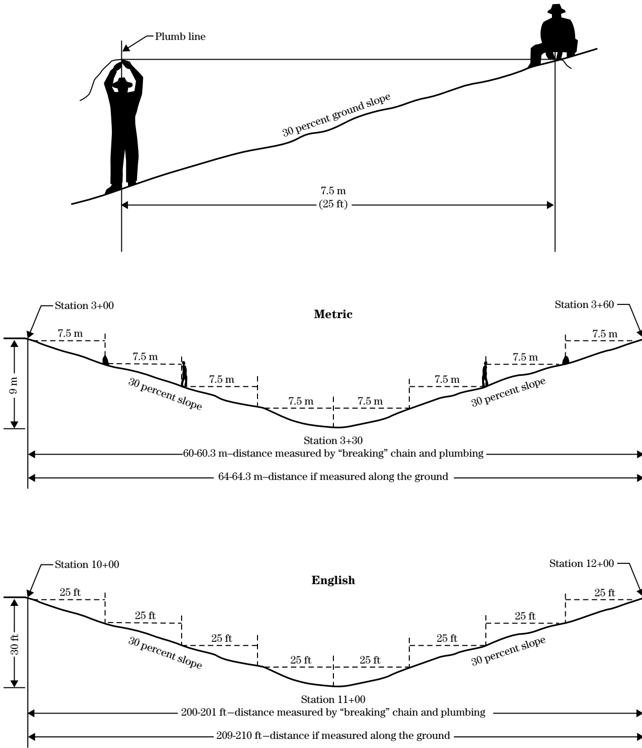
Figure 1-17 Breaking chain
