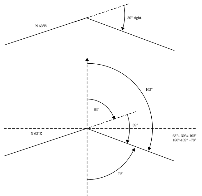
Figure 1-22 Course direction determination from measured angles
