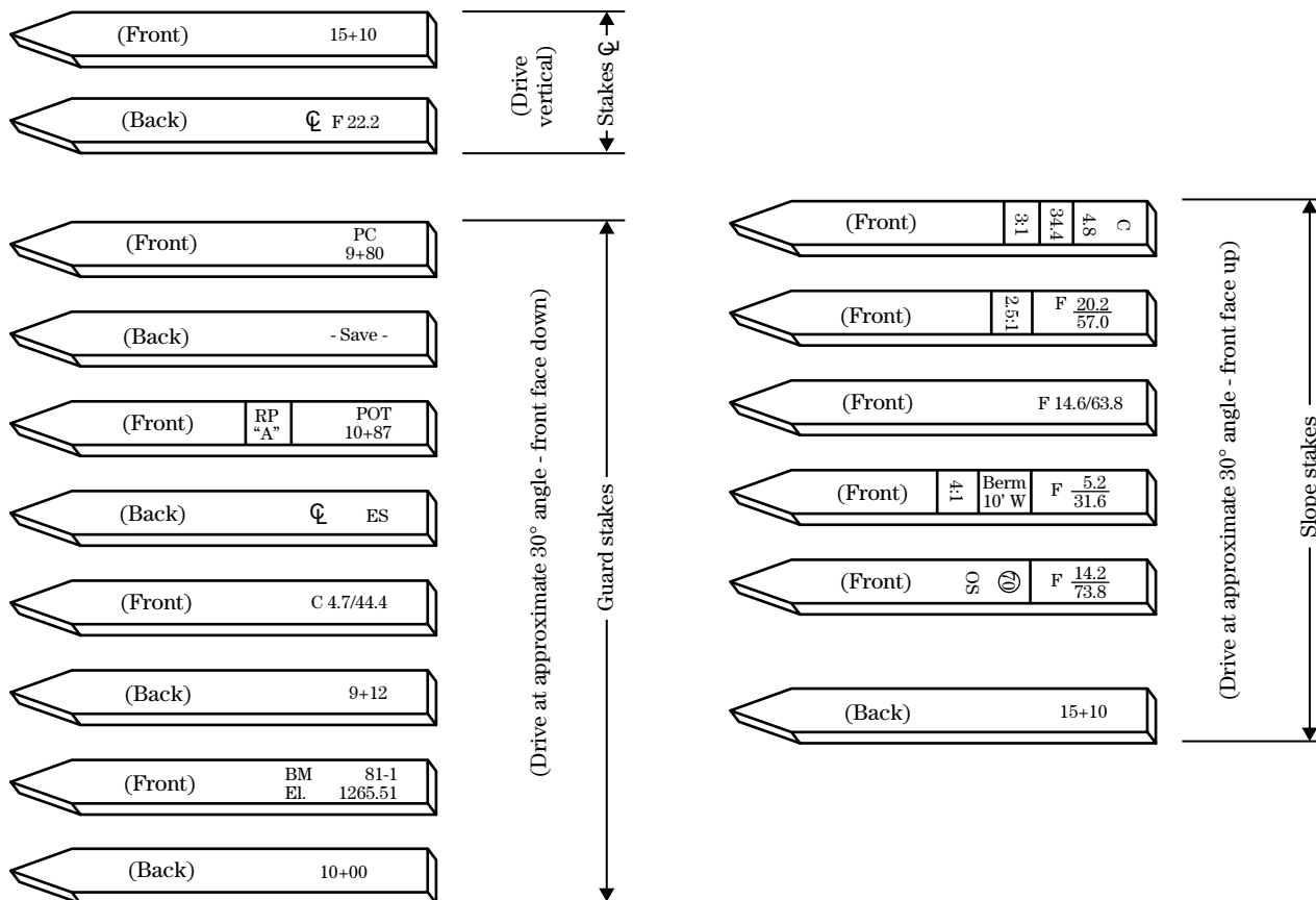
Figure 1-67 Slope stakes
