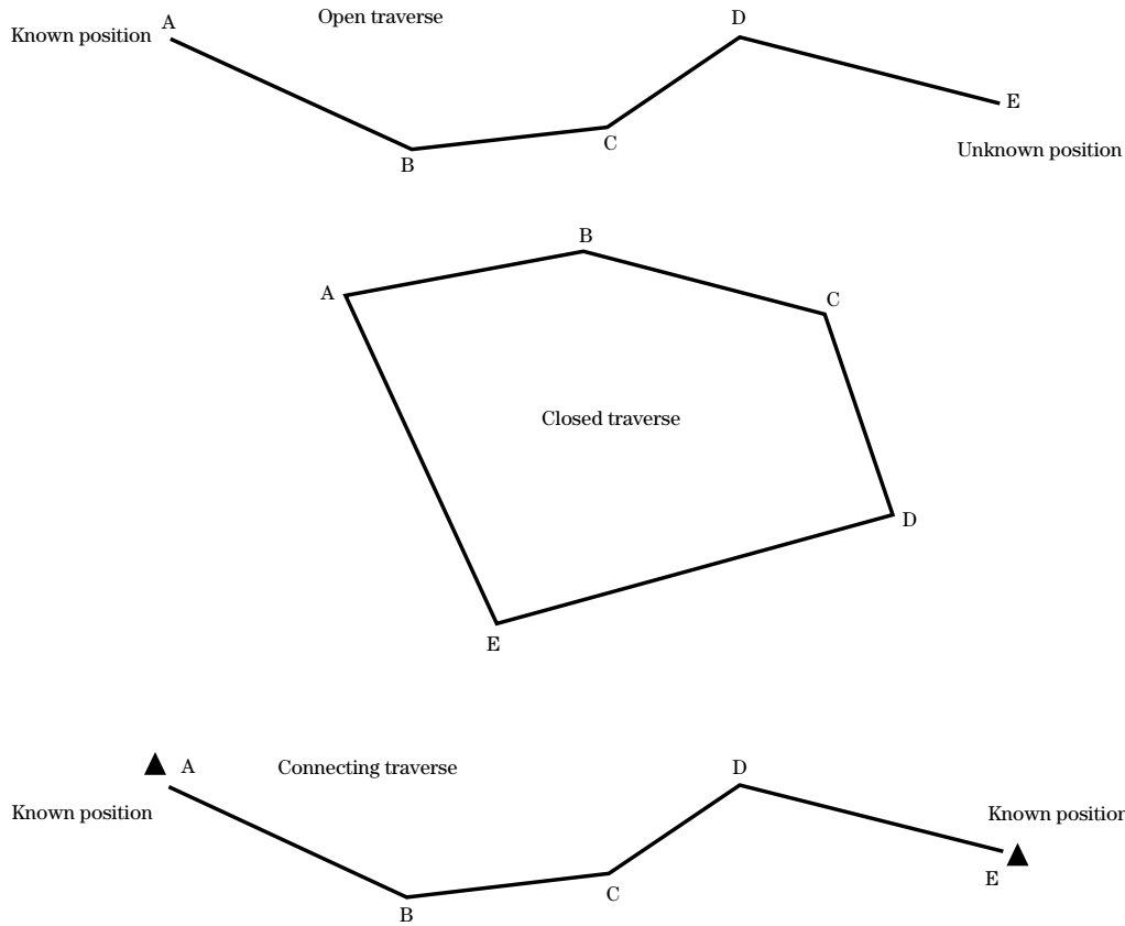
Figure 1-9 Open traverse
