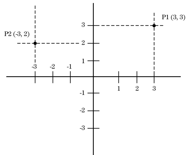
Figure 1-75 Cartesian coordinate system showing the rectangular coordinates of points P1 and P2 with respect to an origin (0, 0). In addition to the rectangular coordinates of each position, the distance and angular position of one point with respect to the other can be determined by simple geometry.
