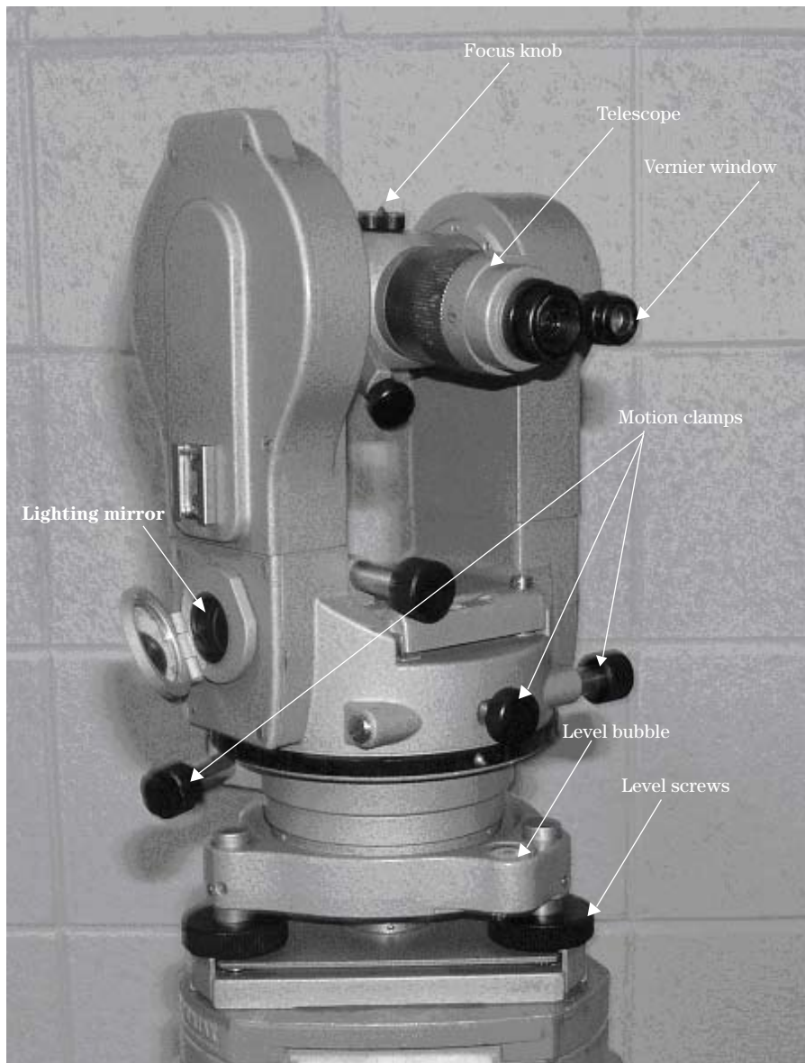
Figure 1-42 Electronic theodolite
