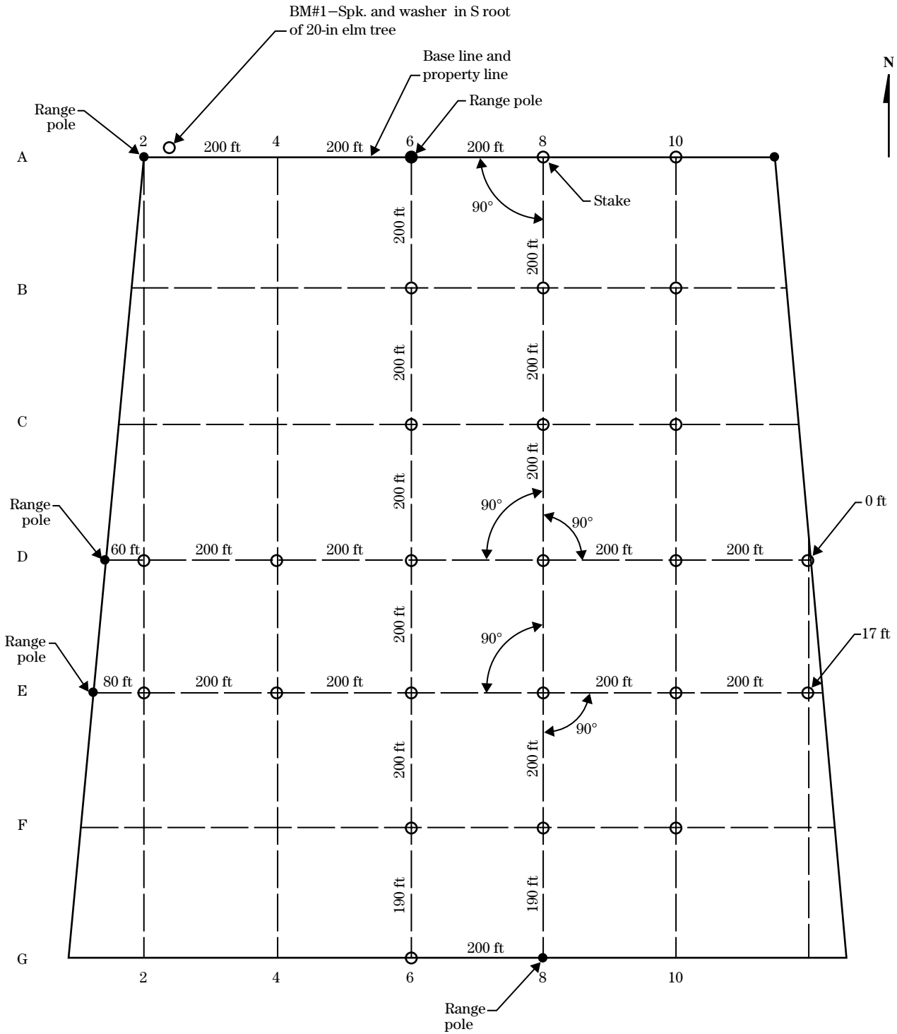
Figure 1-59 Method of topographic survey by gridding
