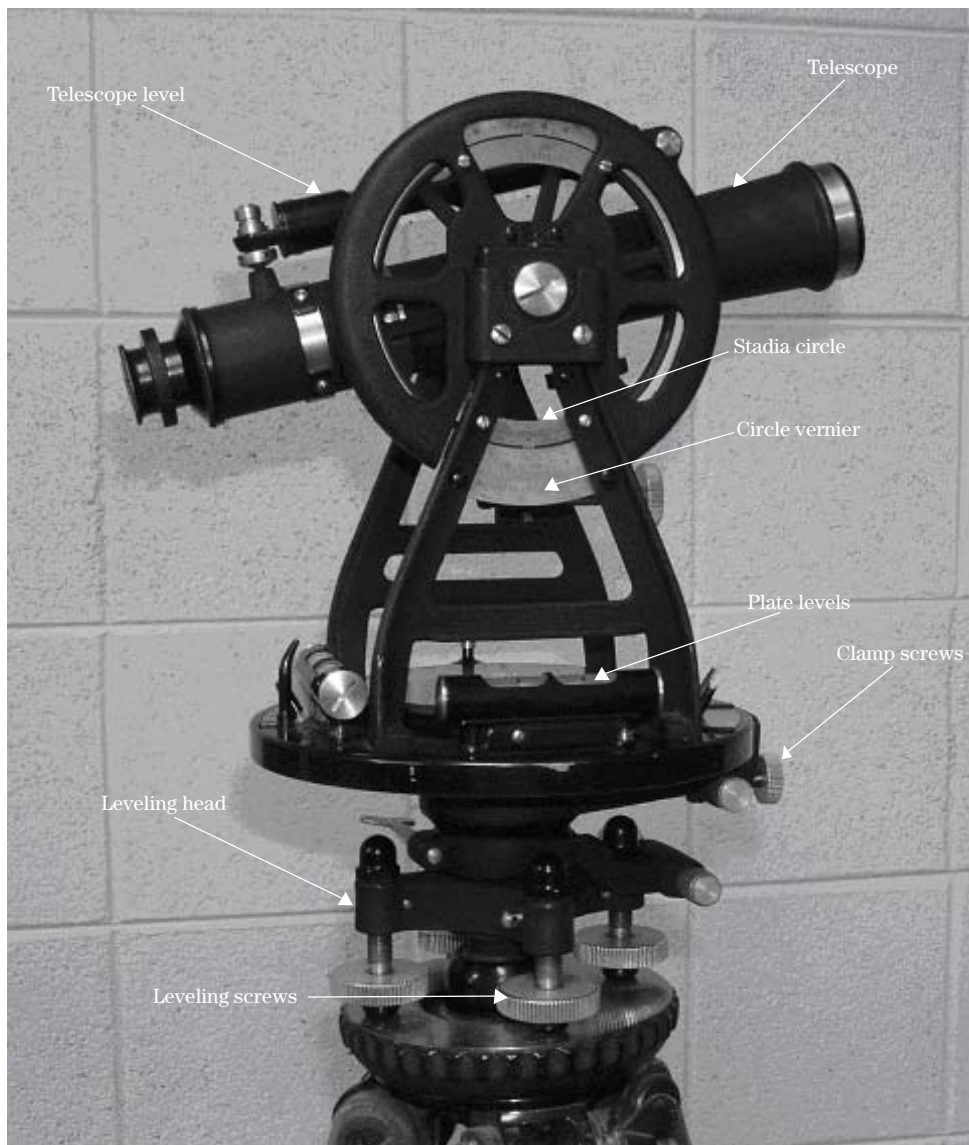
Figure 1-41 Engineer's transit
