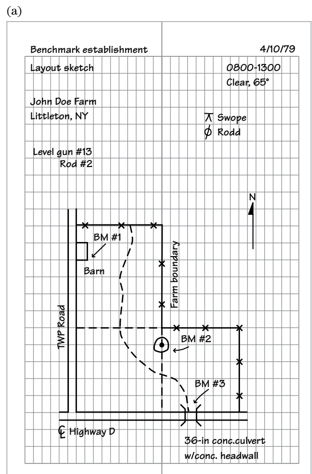
Figure 1–62 Survey notes for a bench level circuit
