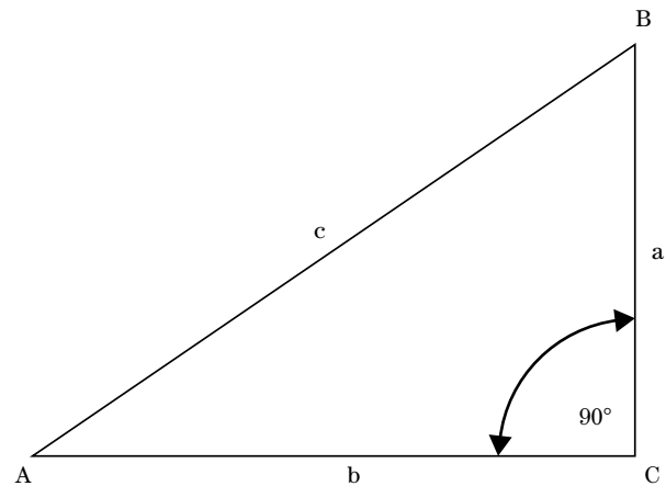
Figure 1-6 Right triangle showing the trigonometric relationships of the lengths of the sides (a,b,c) to the interior angles (A,B,C)
