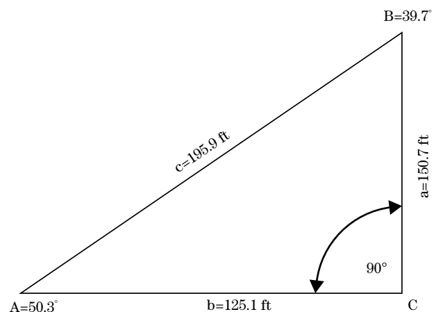
Figure 1-7 Right triangle for table 1-3
