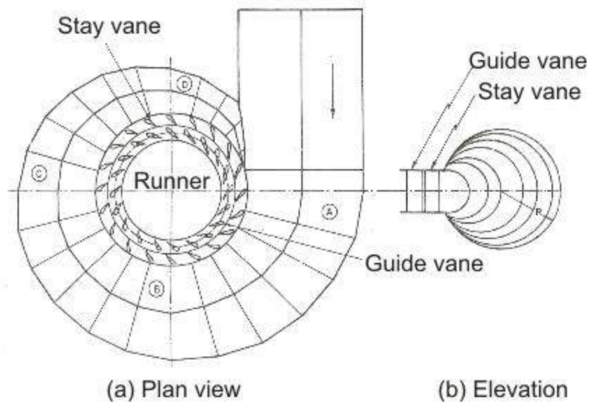
Figure 28.2 Spiral Casing
