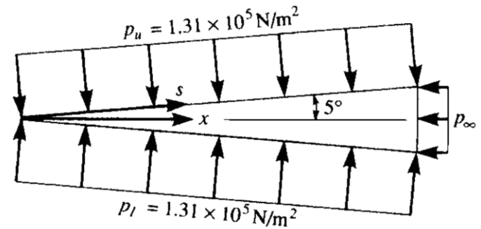
Pressure distribution
