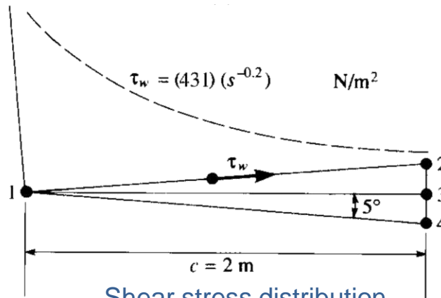
Shear stress distribution
