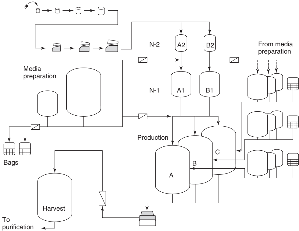
Figure 1.18 Upstream process flow diagram of a design proposal for a 3 \times 10^3 \text{ m}^3 (working volume) monoclonal antibody manufacturing facility. The tanks and bag(s) at the right contain the carbon feed, base, antifoam, and other feeds. The inoculation ratio is 1:4–1:5 in the stirred-tank bioreactors.
