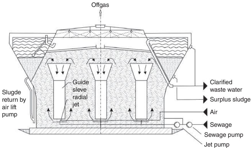
Figure 1.5 Example of an airlift fermenter specifically designed for effective wastewater treatment. This design is the Biohoch Reactor of Hoechst, a jet-loop reactor with multiple internal guide sleeves and a volume of 8000 m 3 .
