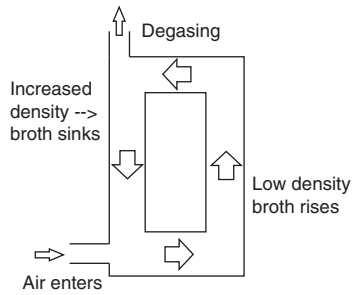
Air lift reactor: pressure cycle disengagement of gas
