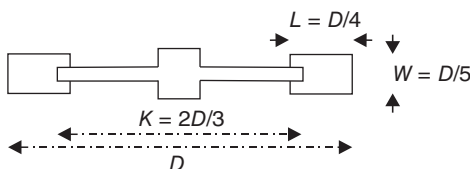
Figure 1.14 Standard design for a Rushton impeller.
