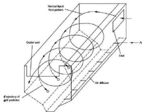
Figure 5.29 Aerated grit chamber
