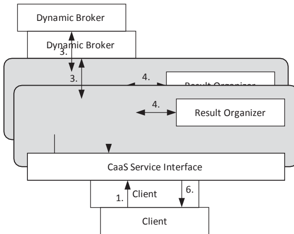
FIGURE 3.6. Cluster discovery.
