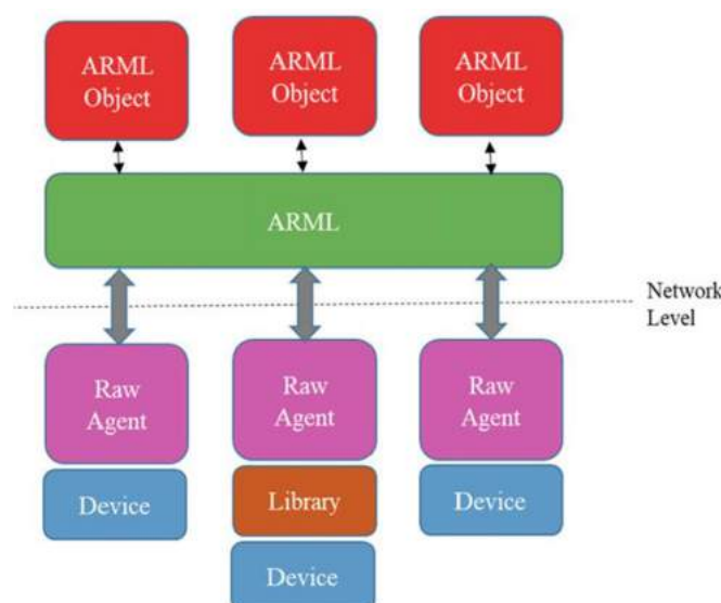
Figure 6. Functional blocks ARML [20].
