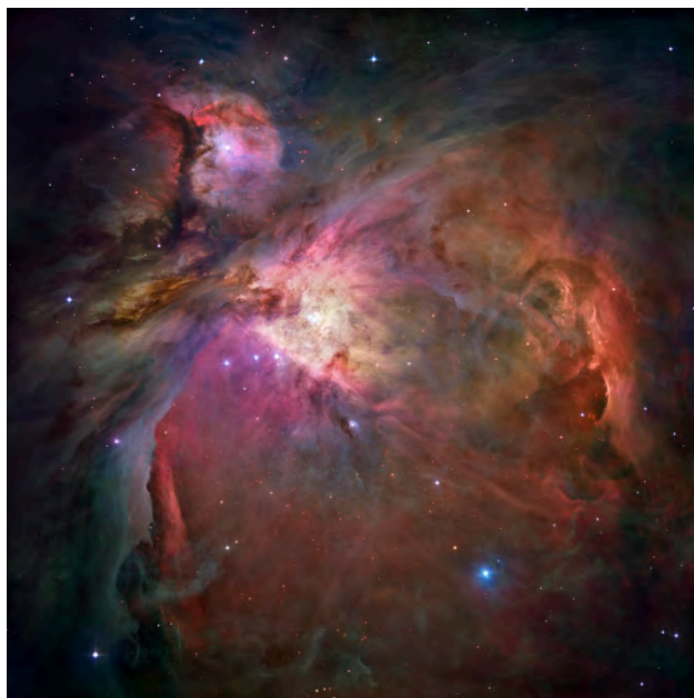
Figure 20.3 Orion Nebula. The red glow that pervades the great Orion Nebula is produced by the first line in the Balmer series of hydrogen. Hydrogen emission indicates that there are hot young stars nearby that ionize these clouds of gas. When electrons then recombine with protons and move back down into lower energy orbits, emission lines are produced. The blue color seen at the edges of some of the clouds is produced by small particles of dust that scatter the light from the hot stars. Dust can also be seen silhouetted against the glowing gas. (credit: NASA,ESA, M. Robberto (Space Telescope Science Institute/ESA) and the Hubble Space Telescope Orion Treasury Project Team)
