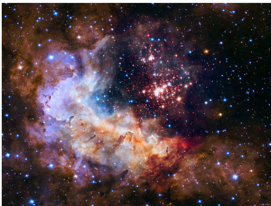
Figure 21.6 Westerlund 2. This young cluster of stars known as Westerlund 2 formed within the Carina star-forming region about 2 million years ago. Stellar winds and pressure produced by the radiation from the hot stars within the cluster are blowing and sculpting the surrounding gas and dust. The nebula still contains many globules of dust. Stars are continuing to form within the denser globules and pillars of the nebula. This Hubble Space Telescope image includes near-infrared exposures of the star cluster and visible-light observations of the surrounding nebula. Colors in the nebula are dominated by the red glow of hydrogen gas, and blue-green emissions from glowing oxygen. (credit: NASA, ESA, the Hubble Heritage Team (STScI/AURA), A. Nota (ESA/STScI), and the Westerlund 2 Science Team)
