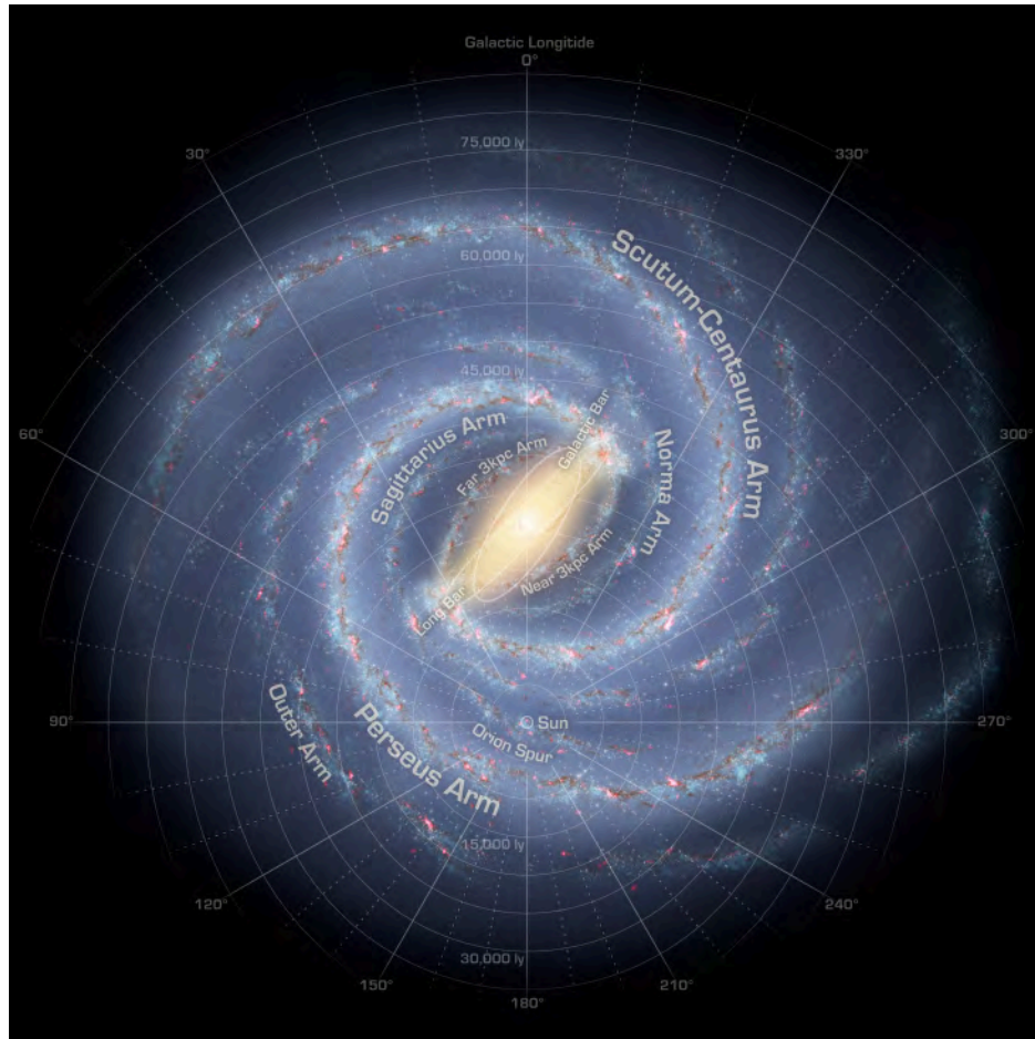
Figure 2 Structure of the Milky Way Galaxy.
