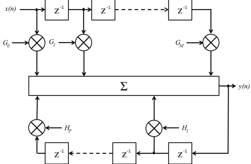
Fig. 24. Physical structure of IIR filter [28]
