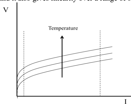
Fig. 5. V-I characteristics of bipolar transistor [7]
