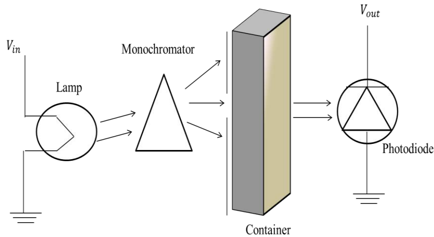
Fig. 9. A simple spectrophotometer [7]
