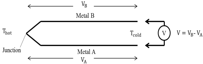
Fig. 2. Working principle of thermocouple [7]
