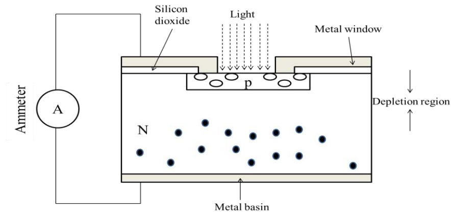
Fig. 7. Photodiode in photovoltaic mode [7]
