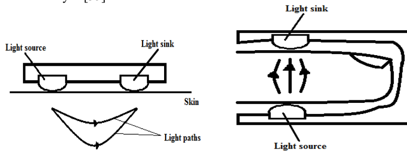
Fig. 39. Reflection mode [35]
