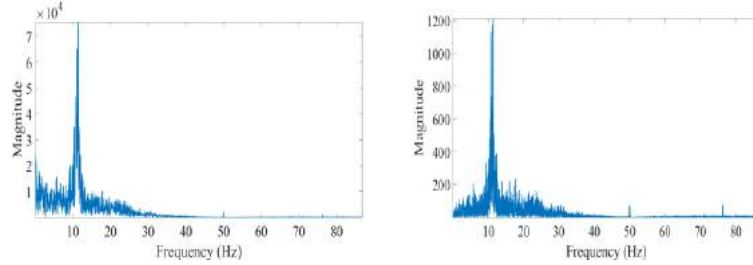
Fig. 21. Magnitude spectrum of Fourier transform Fig. 22. Magnitude spectrum of FBSE
