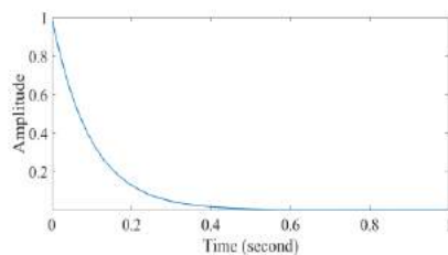
Fig. 14. Aperiodic exponential signal
