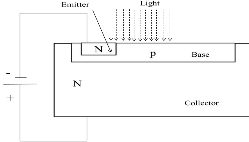
Fig. 8. A NPN phototransistor [7]
