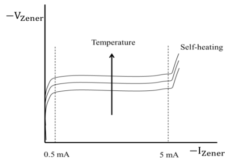
Fig. 4. Reverse bias V-I characteristic of a Zener diode [7]
