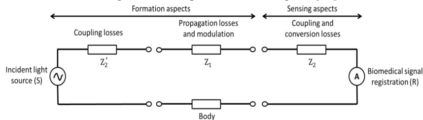
Fig. 37. Electrical model for the registration of induced optic biomedical signal [35]
