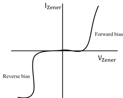
Fig. 3. I-V characteristic of a Zener diode [7]
