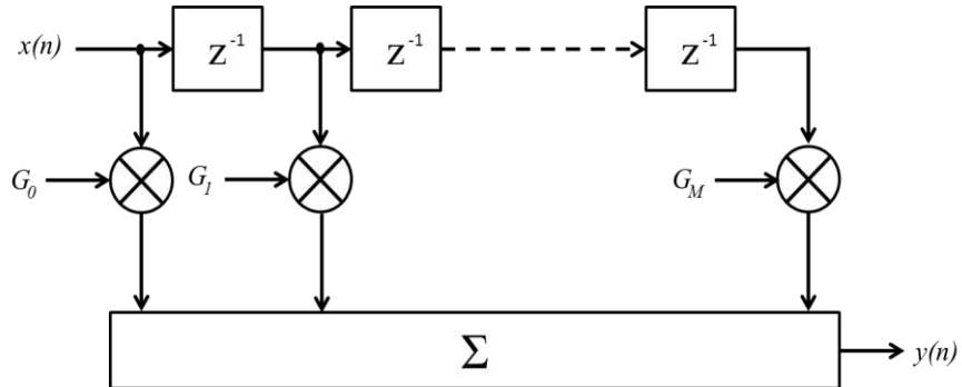
Fig. 23. Physical structure of FIR filter [28]
