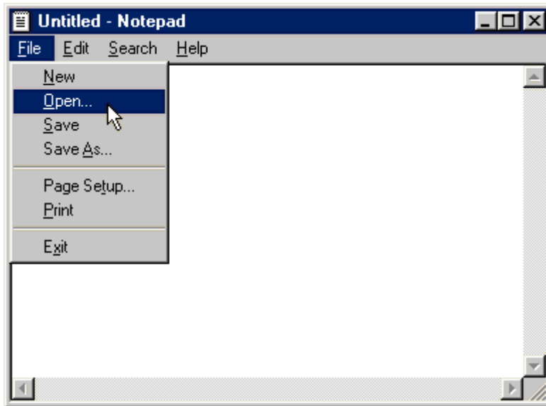
Figure 3: Notepad Environment
