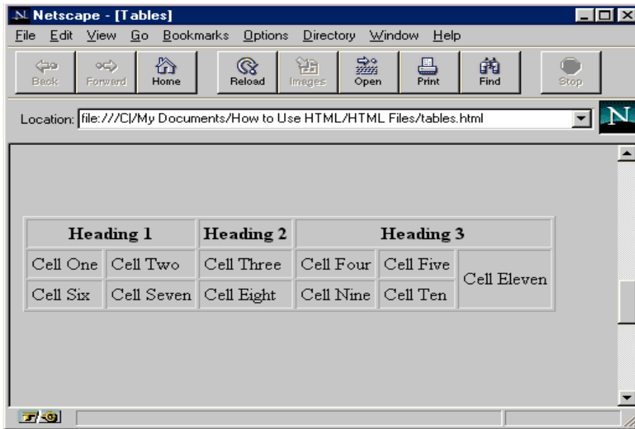
Figure 5: The WIDTH attribute
