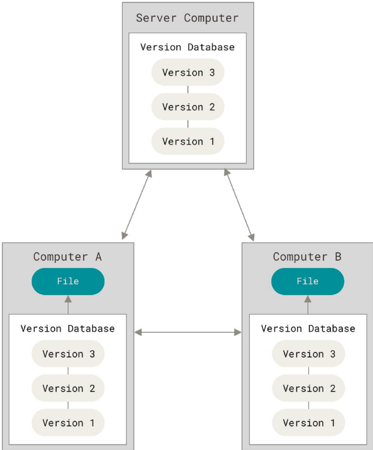
Figure 3. Distributed version control
