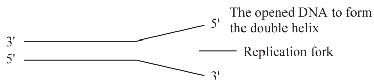
Fig. 23.7a Replication fork
