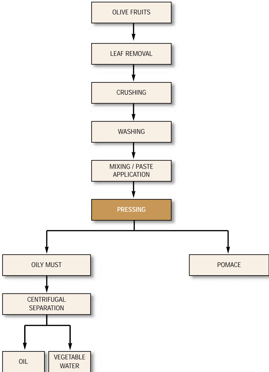
Figure 5.1.2.1. Diagram of olive oil extraction by pressure (A)
