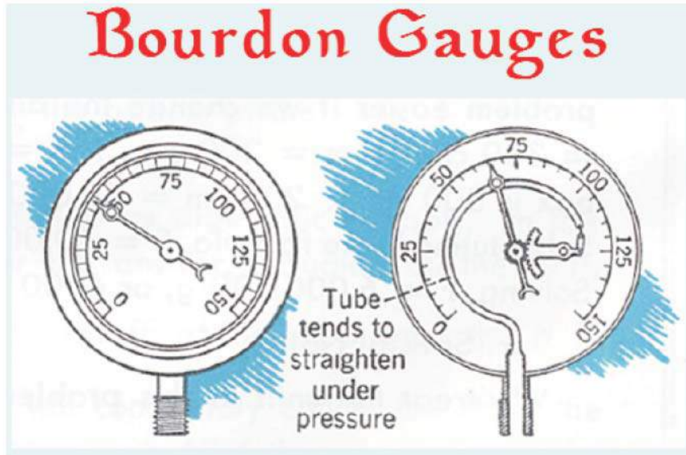
Fig. 11: Bourdon gauge.
