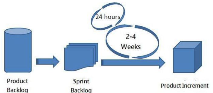
Fig. 7. Scrum process
