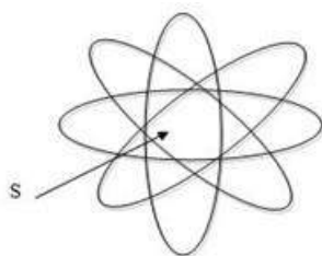
Figure 1. Orbits
