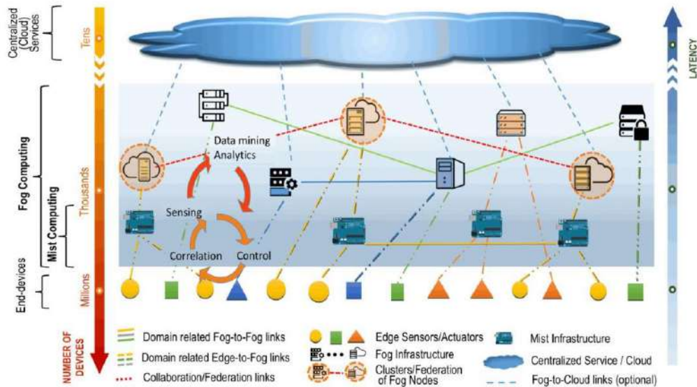
Figura 15 Fod Computing
