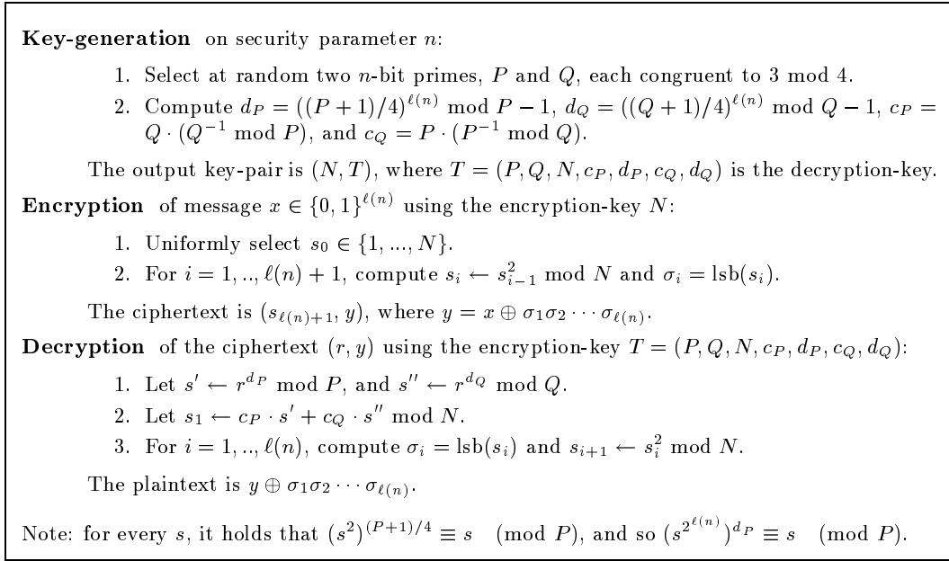
Figure 2: The Blum–Goldwasser Public-Key Encryption Scheme [18]. For simplicity we assume that \ell , which is polynomially bounded (e.g., \ell(n) = n ), is known at key-generation time.
