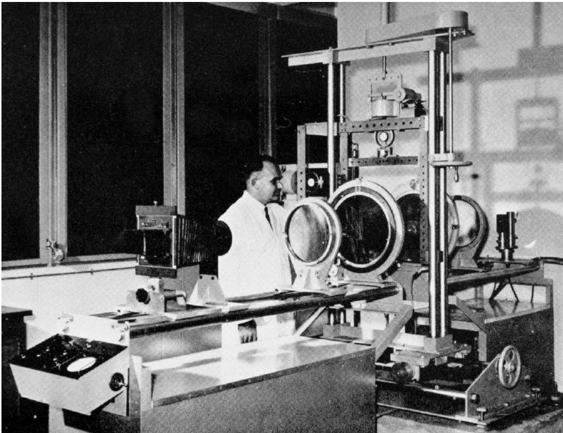
Figure 1. The C.S.I.R. polariscope for producing a 12 in.diameter beam of polarised light for photoelastic model analysis.
