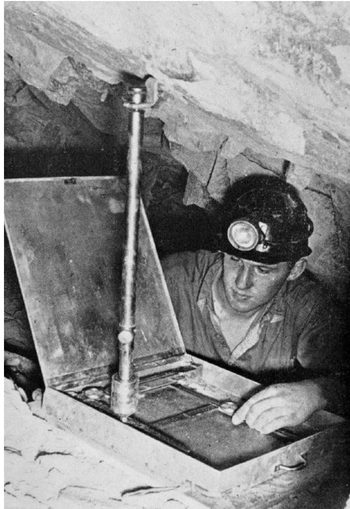
Figure 5. An instrument used by the South African C.S.I.R. for the measurement of closure and ride in a slope in a deep-level gold mine.
