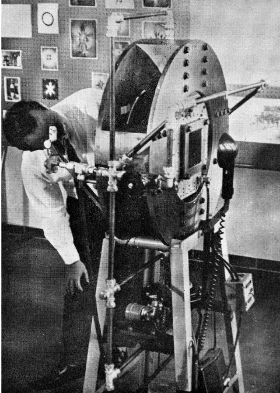
Figure14. Apparatus used by the C.S.I.R. for subjecting plate models to biaxial compressive loading.
