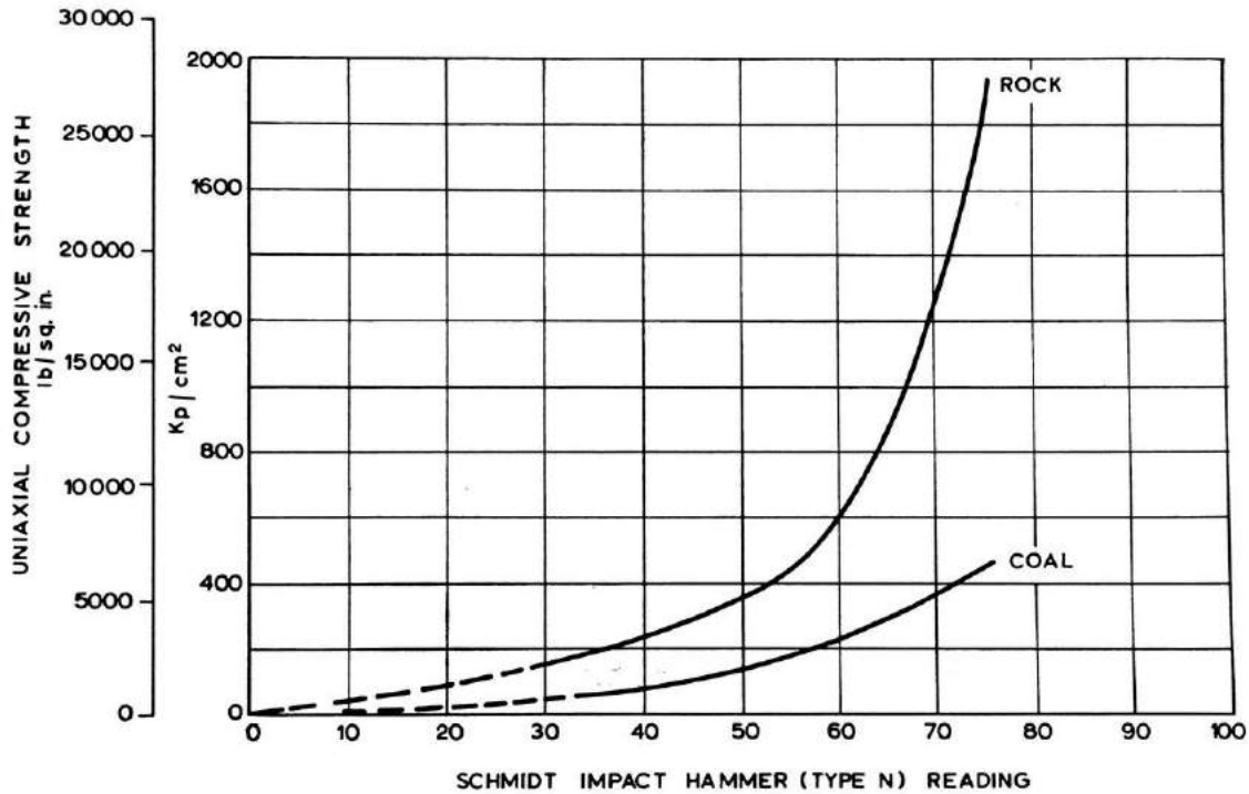
Figure 10. Relationship between the uniaxial compressive strength of rock and the Schmidt impact hammer reading (according to Skutta).
