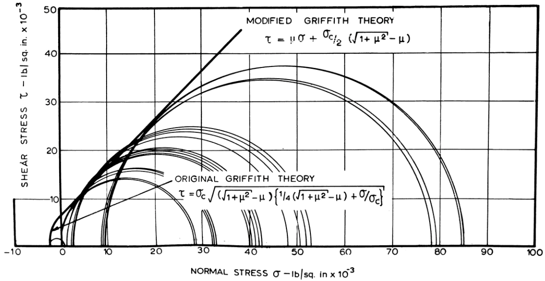
Figure 3. Mohr fracture diagram for typical Witwaterstrand quartzite with a uniaxial compressive strength \sigma_c = 30,000 p.s.i. and a coefficient of internal friction \mu = 1.00
