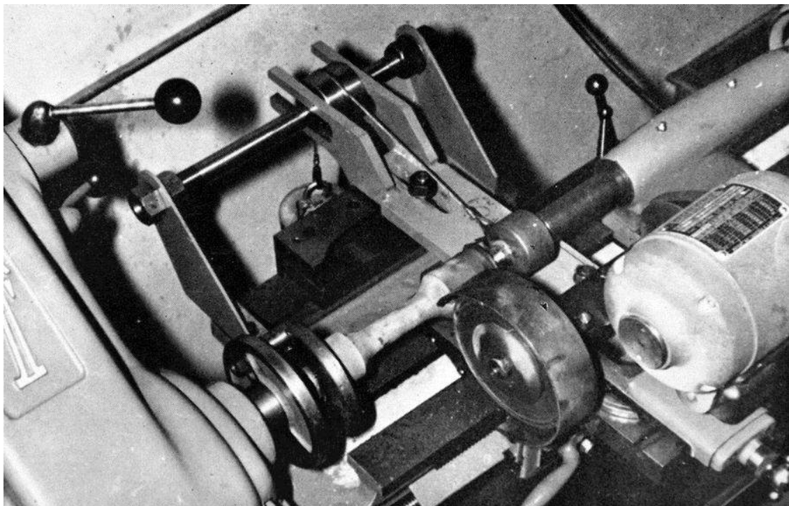
Figure 9. Apparatus for the preparation of tensile specimens in the laboratories of the South African C.S.I.R.
