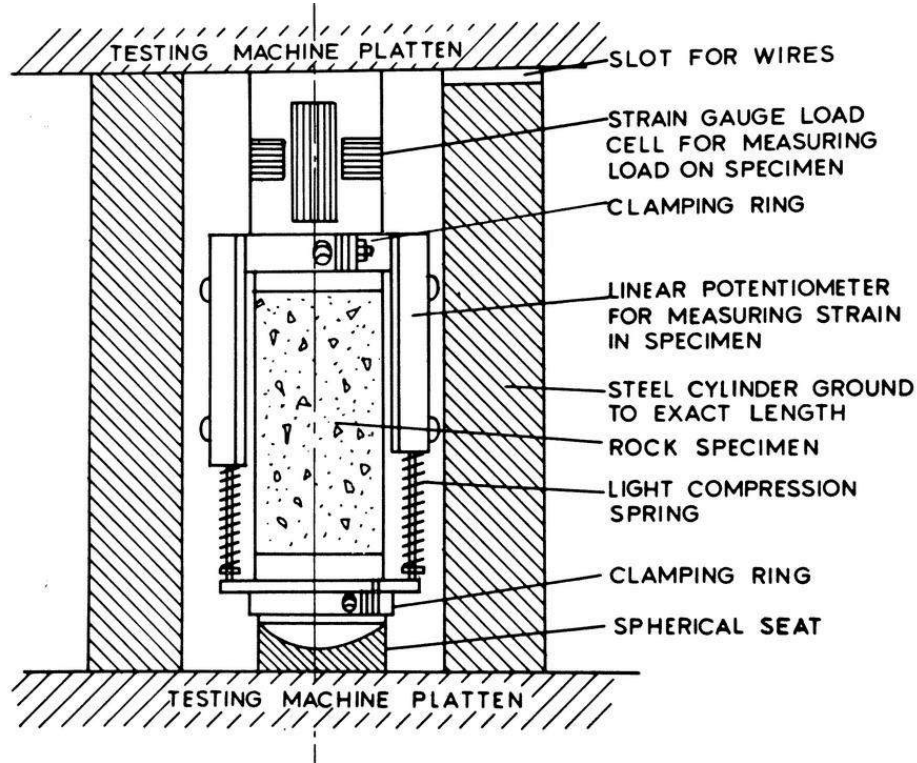
Figure 13. Apparatus for tests to simulate load transfer from a specimen at point of failure.
