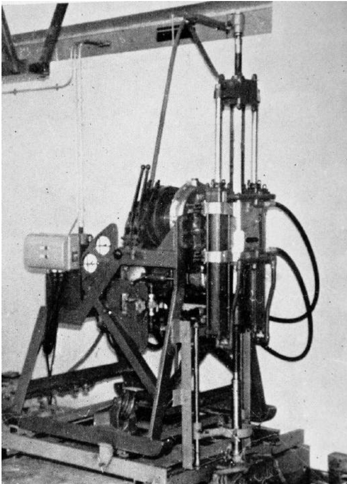
Figure 7: Drilling machine used to obtain specimens in the laboratories of the South African C.S.I.R.
