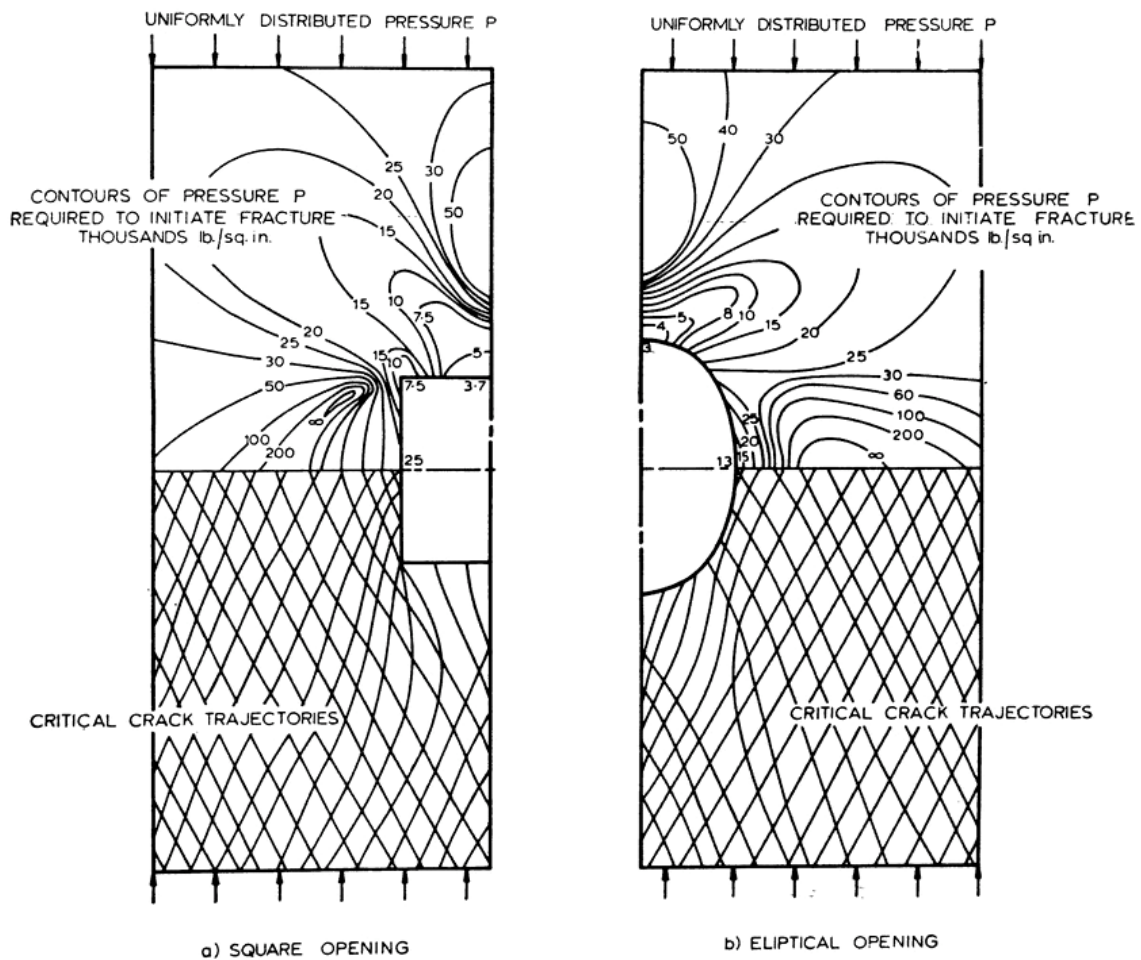
Figure 8. Fracture contours and critical crack trajectories in quartzite surrounding square and elliptical tunnels
