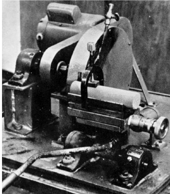
Figure 8: Machine used by the C.S.I.R. for grinding the ends of cylindrical specimens.
