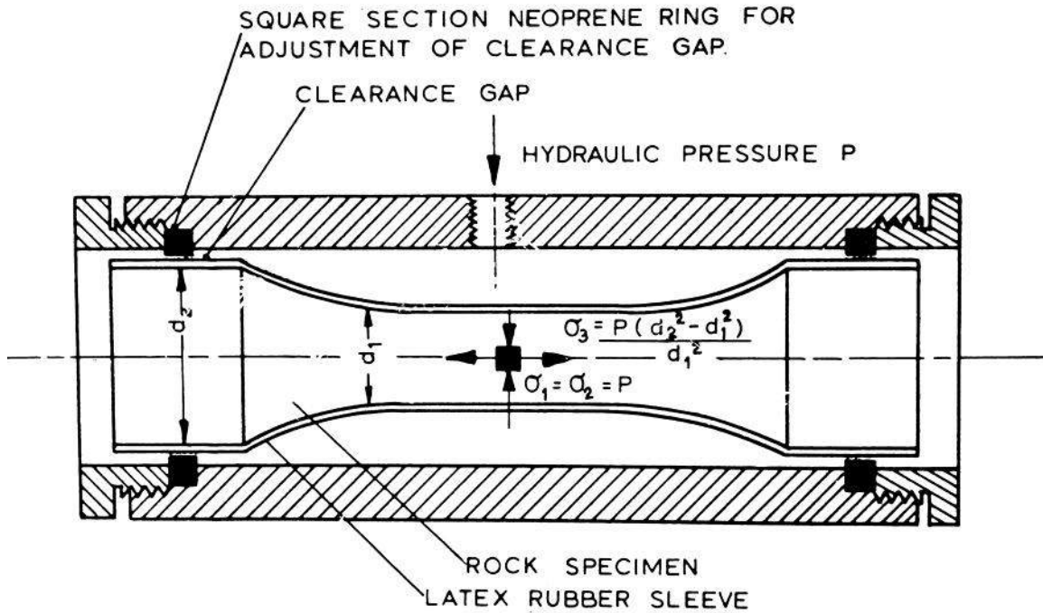
Figure 12. Apparatus for determining the tensile strength of rock specimens.
