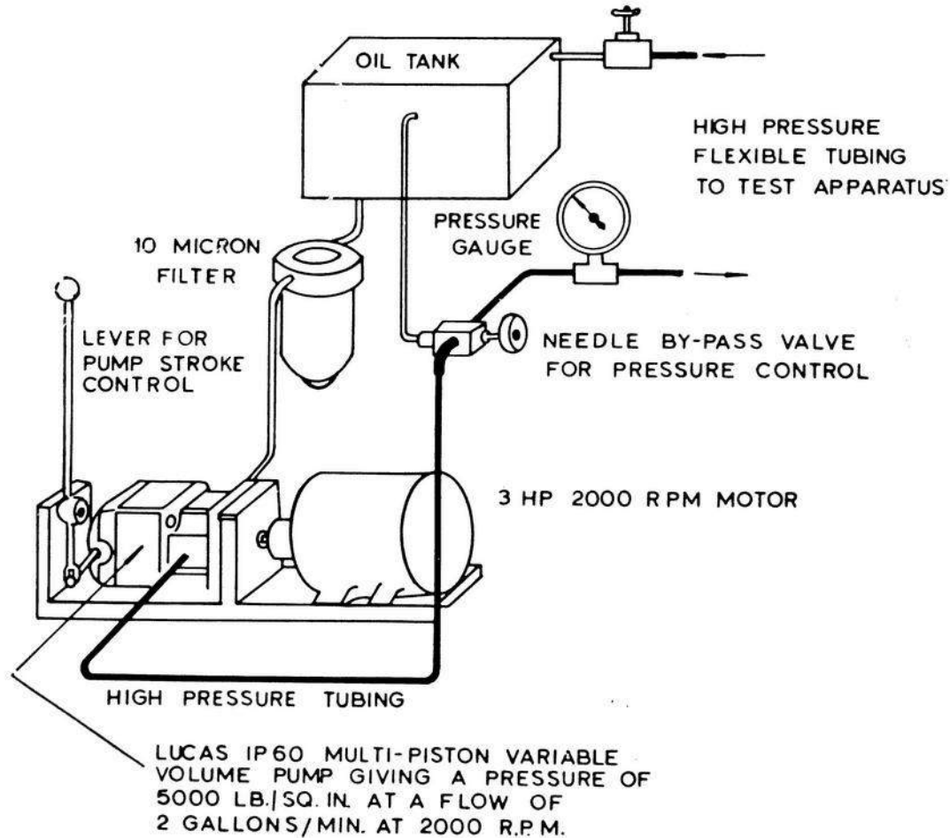
Figure 11. Circuit used for producing accurately controlled hydraulic pressures.
