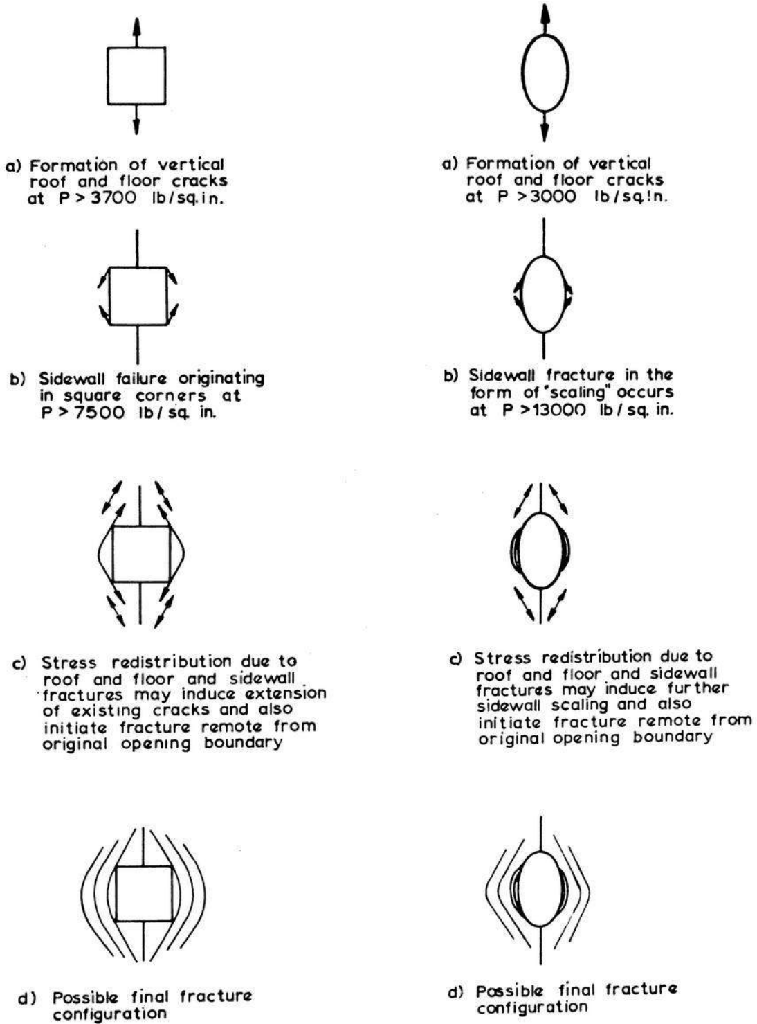
Figure 9. Possible fracture sequence for square and elliptical tunnels in hard quartzite subjected to vertical pressure P only
