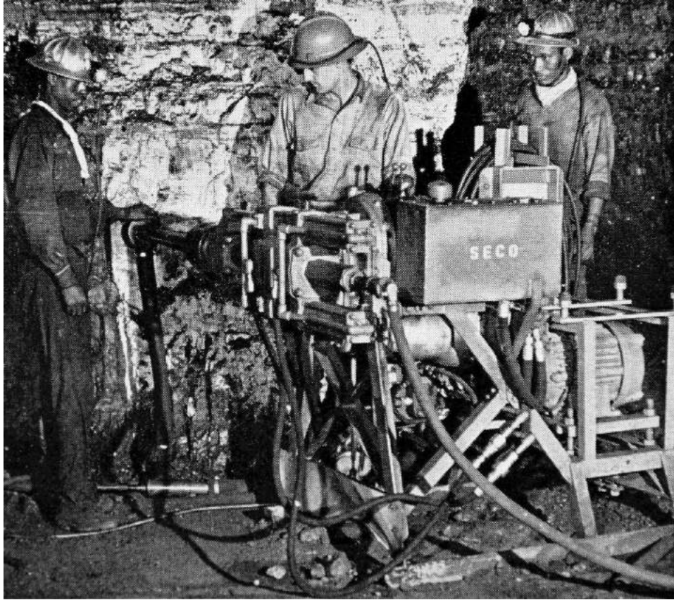
Figure 7. Drilling coal specimens for properties testing
