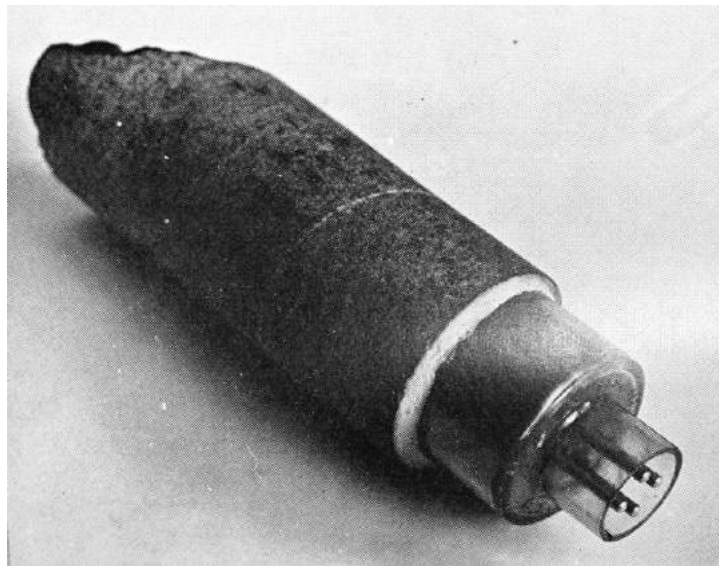
Figure 2. A C.S.I.R. Strain cell bonded on to a rock core recovered from a borehole.
