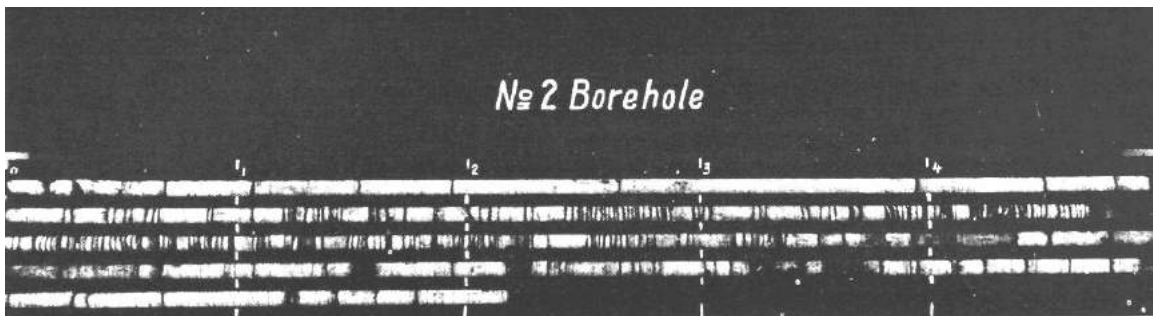
Figure 4. Disking of core recovered from a borehole drilled into highly stressed rock.
