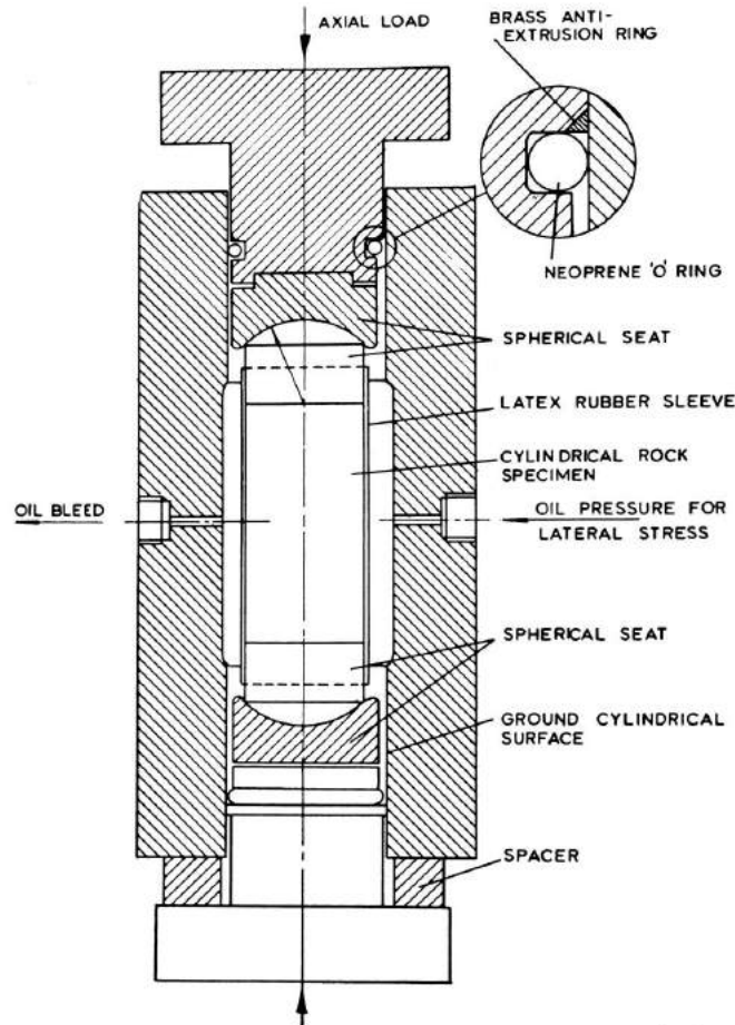
Figure 10. Apparatus for subjecting cylindrical rock specimens to triaxial compressive stress conditions.
