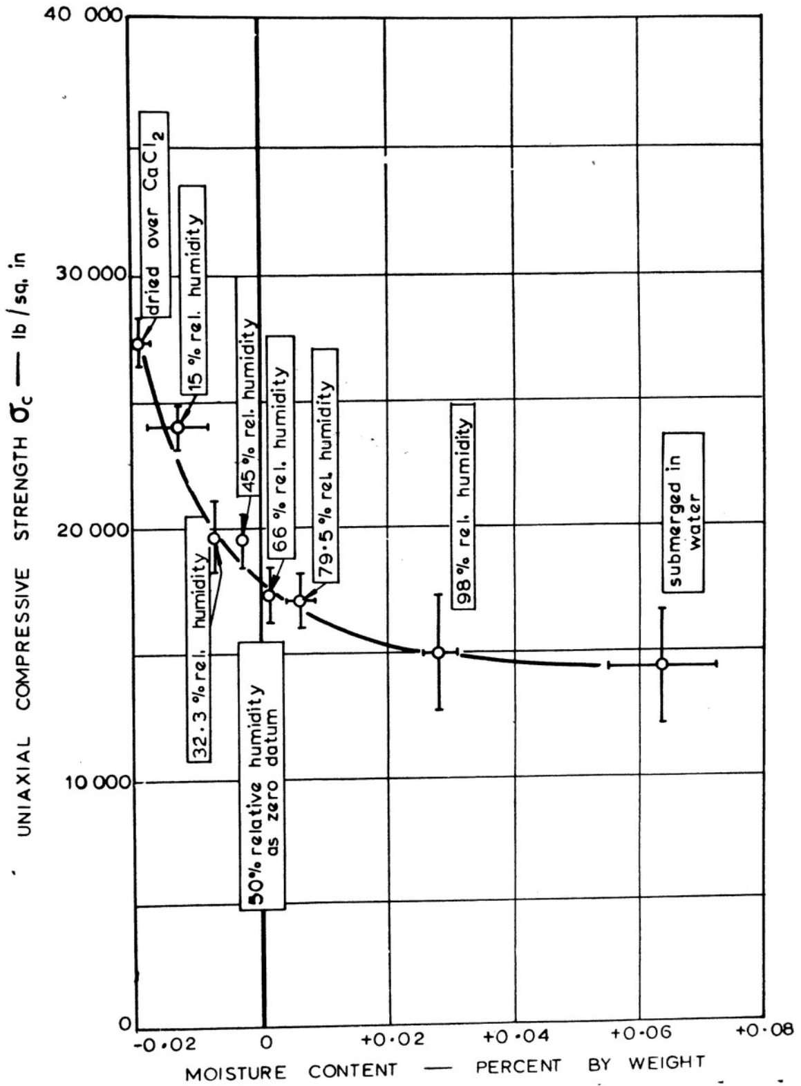
Figure 5. Relationship between uniaxial compressive strength and moisture content for quartzitic shale specimens (Colback & Wiid).
