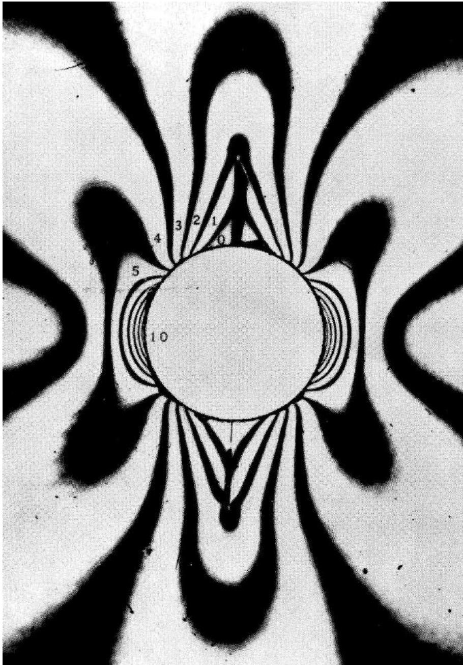
Figure 4. Photoelastic pattern in a glass plate model containing a central circular hole from which vertical tensile cracks have propagated.
