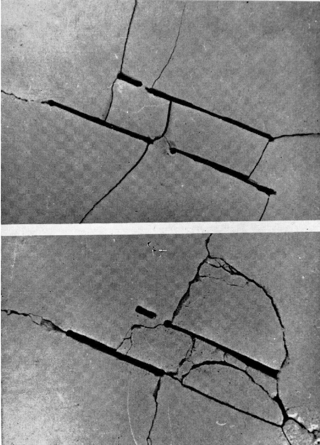
Figure 16. Comparison between the propagation of fracture in plaster of paris models subjected to uniformly distributed edge loading (upper photograph) and centrifugal acceleration (lower photograph).
