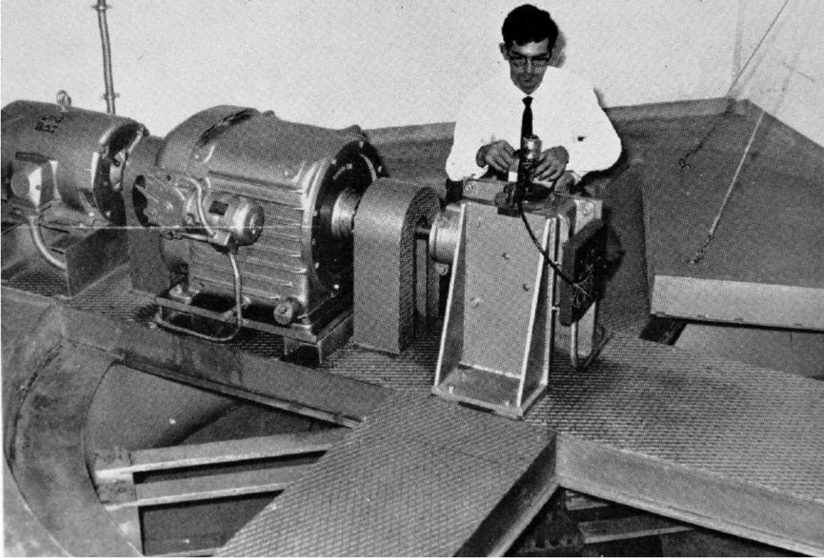
Figure 5. The C.I.S.R.'s 9 ft. diameter centrifuge for subjecting models to acceleration of up to 1,000 times the acceleration due to gravity.
