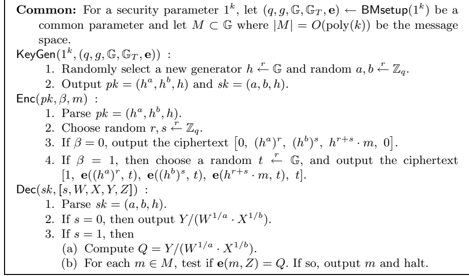
Fig. 1. Encryption Scheme II
