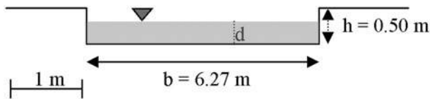
Fig. 22 The Otolum in an open channel
