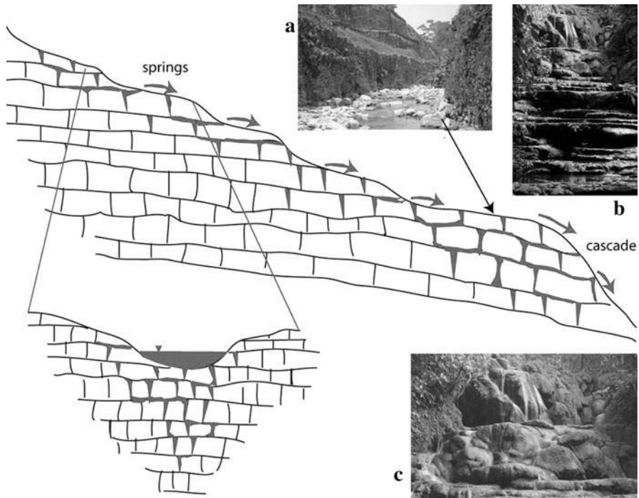
Fig. 3 Hydrologic conceptual model for the Cretaceous limestone watershed at Palenque showing the increased dissolution along bedding planes and fractures below the stream channel bed, a boulder channel ( top photo ) crossing the ruins, and two photos within the groundwater discharge zone showing the pool and ledge cascade and accreting tufa deposits
