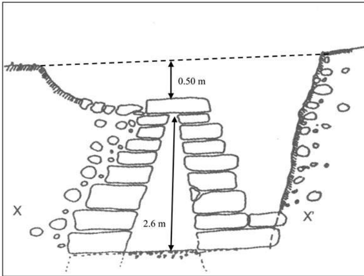
Fig. 21 Cross section of OT-A1's Section C. This is the section that was used to determine the flow rate
