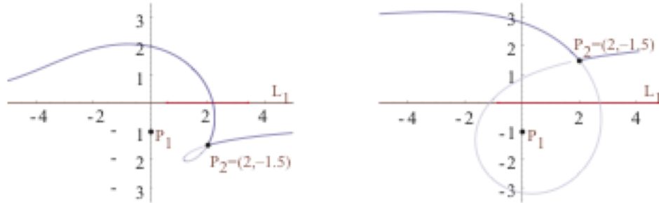
Figure 35. Locus of points swept out by P_2 as the fold line parameter a_f varies from -1 to 1 for two points P_2 .
