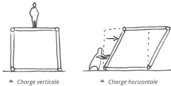
△ Charge verticale
