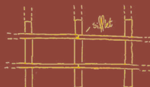
Pannes continues
