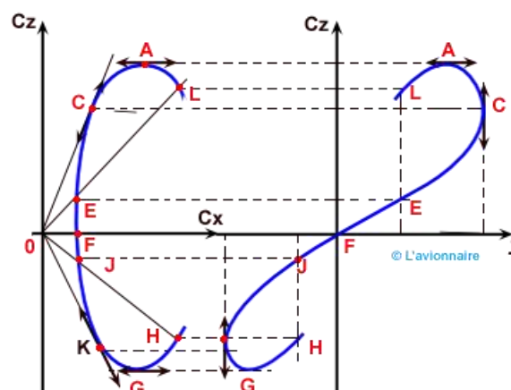
Figure 5.28. La finesse
