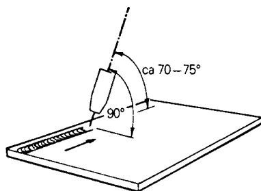
Forehand technique
