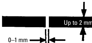
Close square butt joint
