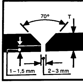
T = 5 - 24 mm V-groove with root
