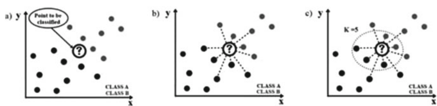
Fig. 10.2 K-nearest Neighbor algorithm (Pacheco et al. 2021)
