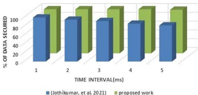
Fig. 10.3 Data security
