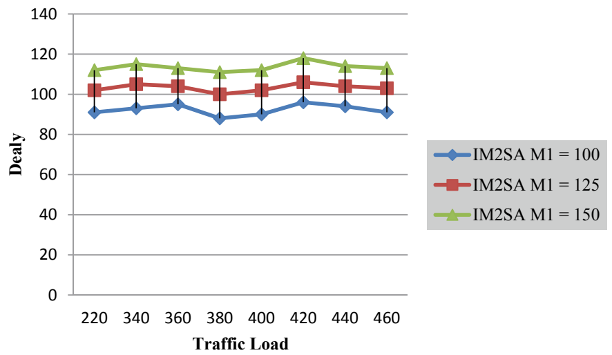
Fig. 4.3 IM2SA delay jitter results (high traffic load)
