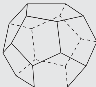
Dodecaedro regular
