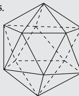
Icosaedro regular
