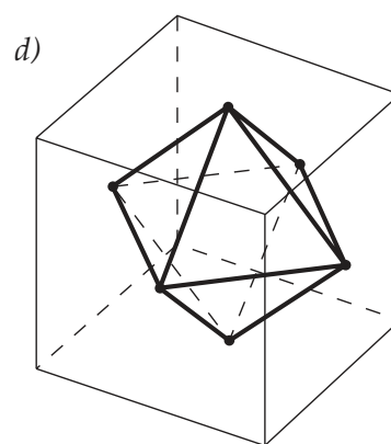
Octaedro regular
