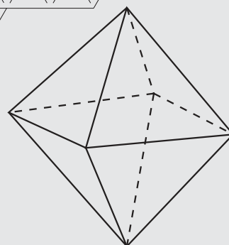
Octaedro regular
