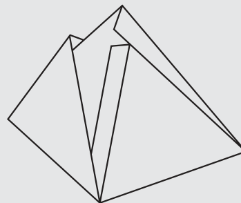
Tetraedro regular
