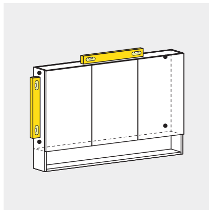
Mirror Cabinets & Wall Cabinets: Ensure cabinet is level and plumb. Mount to wall studs with included screws in each corner.
