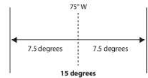
Figure 1.8 Diagram Illustrating the Width of a Time Zone
