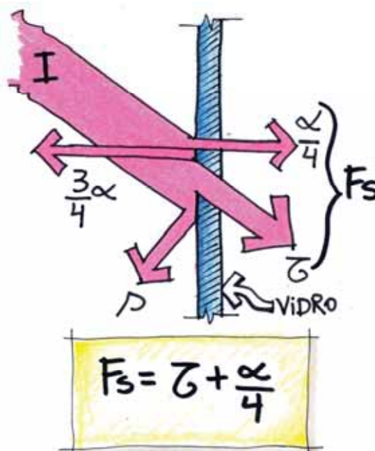
Figura 7-24: Fator solar
