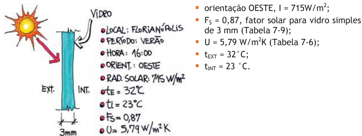
Figura 7-25: Fator solar
